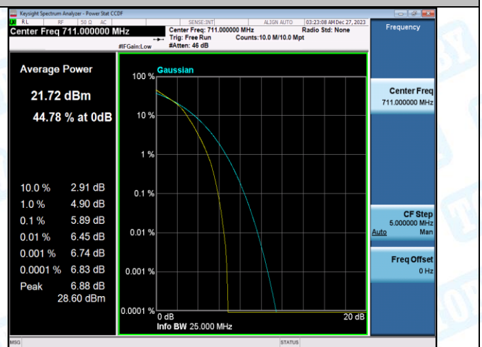
Band12-10MHz-16QAM-23130-50RB#0-PASS
