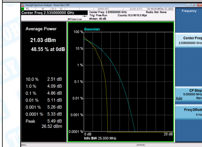
Band7-20MHz-QPSK-21100-100RB#0-PASS
