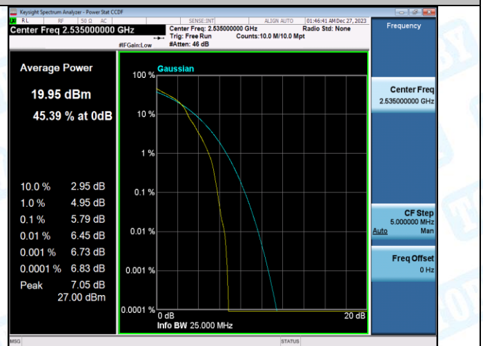
Band7-20MHz-16QAM-21100-100RB#0-PASS
