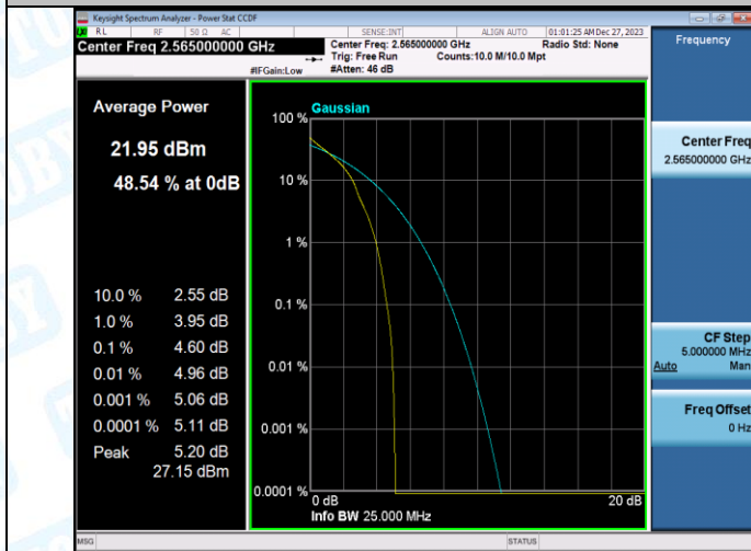
Band7-10MHz-QPSK-21400-50RB#0-PASS
