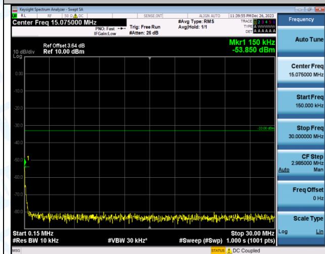
Band4_5MHz_16QAM_20375_1RB#0_1000~3000_1000~3000
