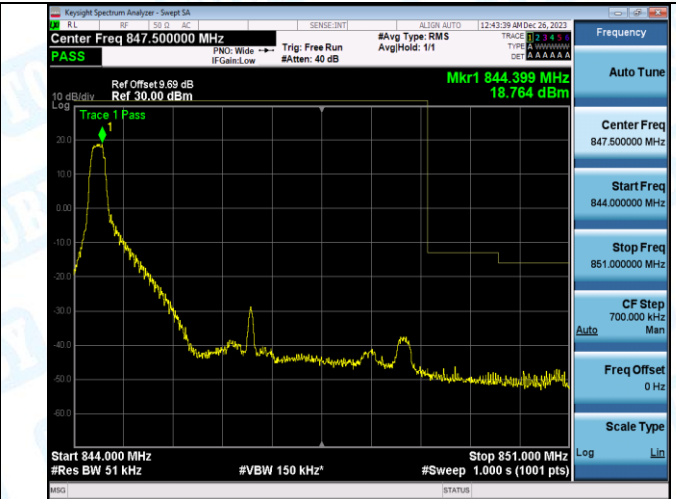
Band5_5MHz_16QAM_20625_1RB#24
