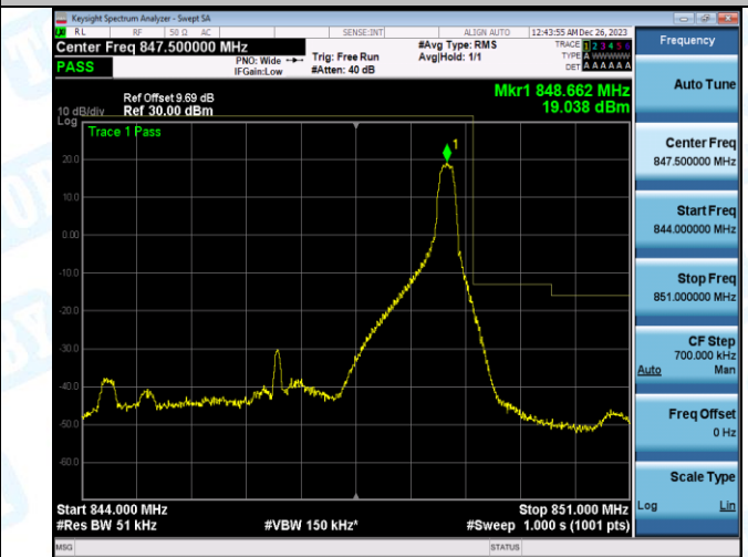
Band5_5MHz_16QAM_20625_25RB#0
