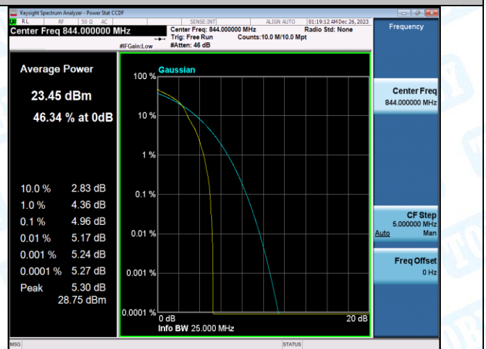
Band5-10MHz-16QAM-20600-50RB#0-PASS
