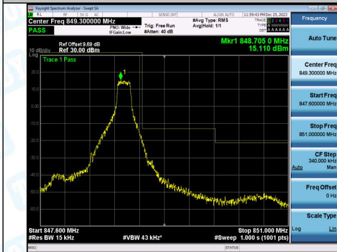
Band5_1.4MHz_QPSK_20643_6RB#0
