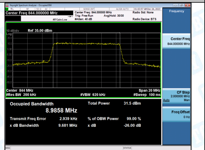
Band5-10MHz-16QAM-20600-50RB#0-PASS
