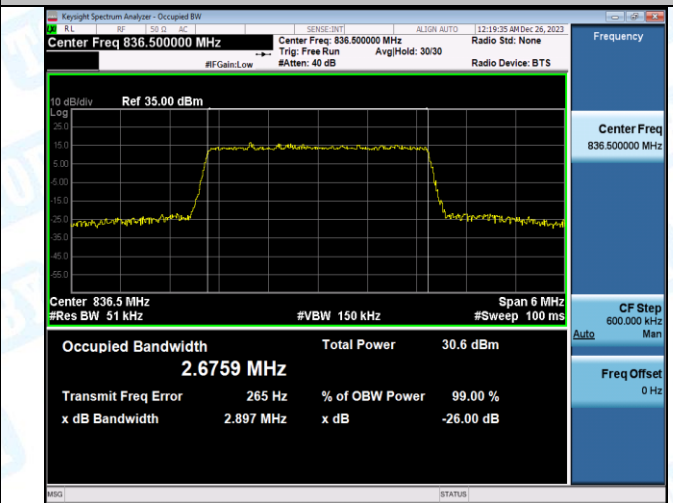
Band5-3MHz-16QAM-20635-15RB#0-PASS
