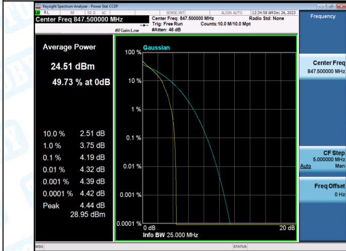
Band5-3MHz-QPSK-20635-15RB#0-PASS
