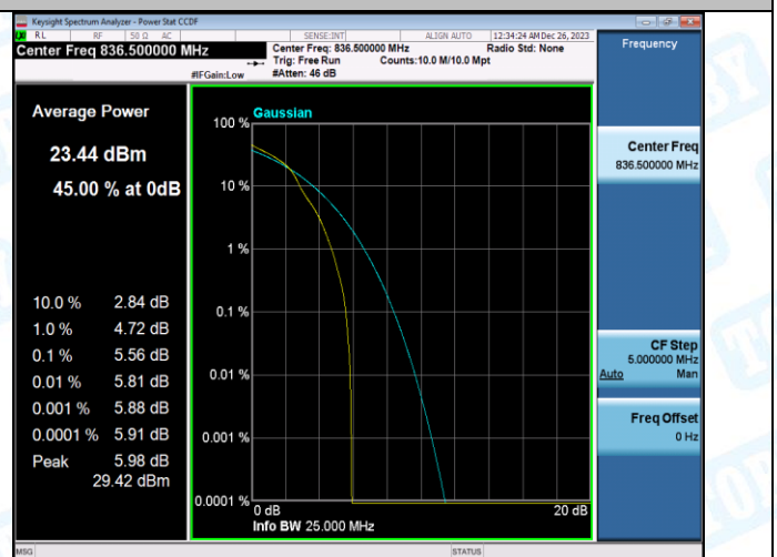
Band5-3MHz-16QAM-20525-15RB#0-PASS
