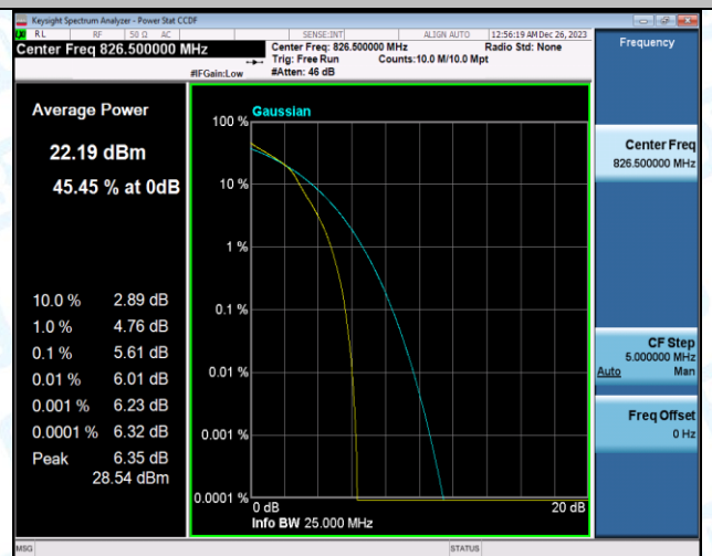
Band5-5MHz-16QAM-20525-1RB#0-PASS
