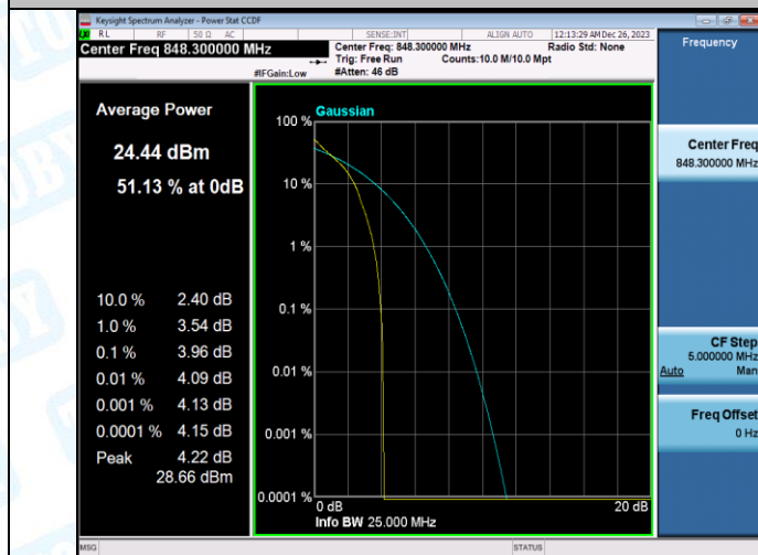
Band5-1.4MHz-QPSK-20643-6RB#0-PASS
