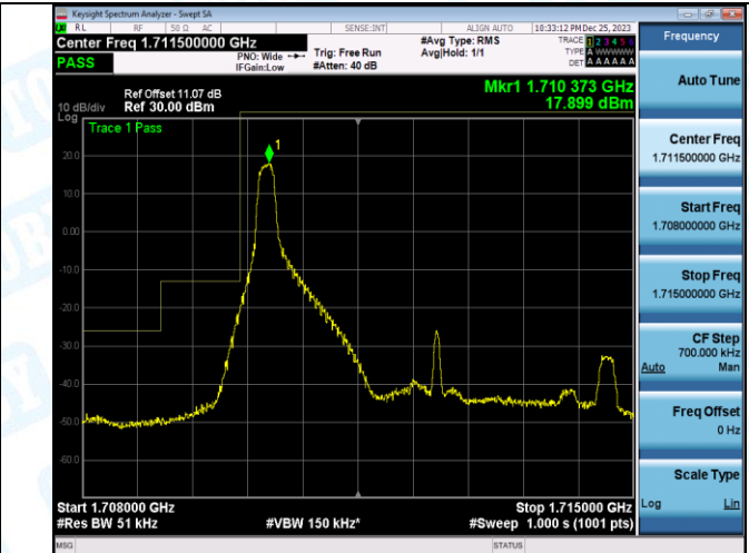
Band4_5MHz_16QAM_19975_1RB#24
