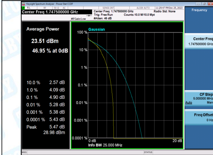
Band4-15MHz-QPSK-20325-75RB#0-PASS
