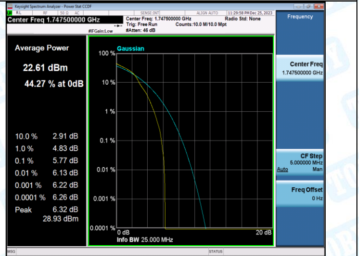
Band4-15MHz-16QAM-20325-75RB#0-PASS
