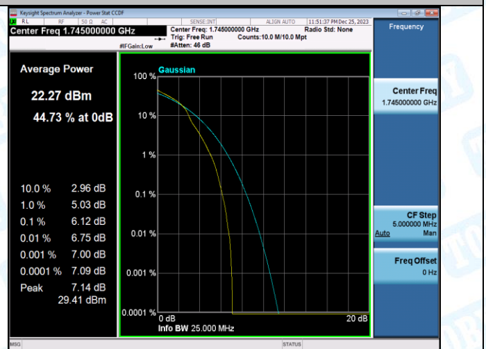
Band4-20MHz-16QAM-20300-100RB#0-PASS
