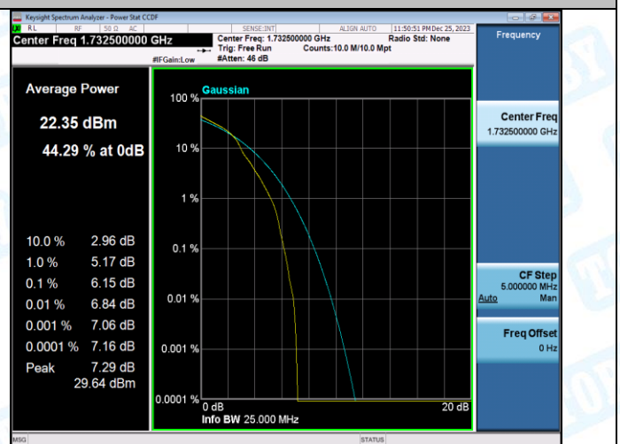
Band4-20MHz-16QAM-20175-100RB#0-PASS
