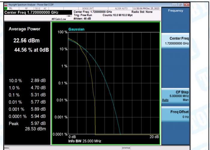
Band4-20MHz-16QAM-20050-100RB#0-PASS
