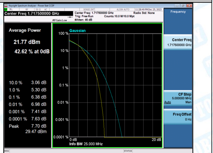
Band4-15MHz-16QAM-20175-1RB#0-PASS
