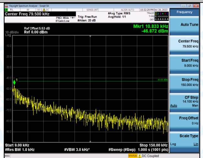
Band2_3MHz_16QAM_18900_1RB#0_30~1000_30~1000
