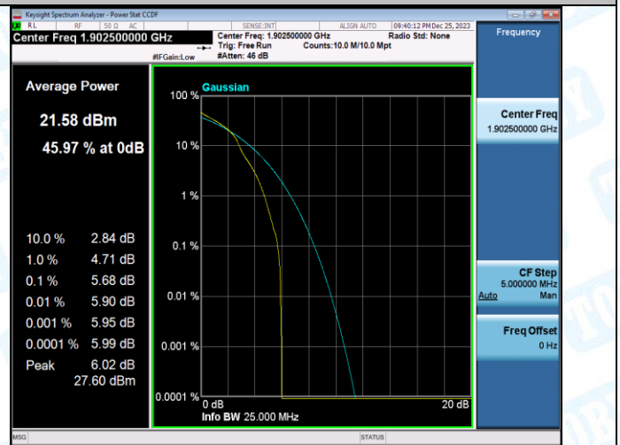
Band2-15MHz-16QAM-19125-75RB#0-PASS
