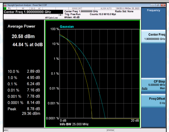
Band2-20MHz-16QAM-19100-100RB#0-PASS
