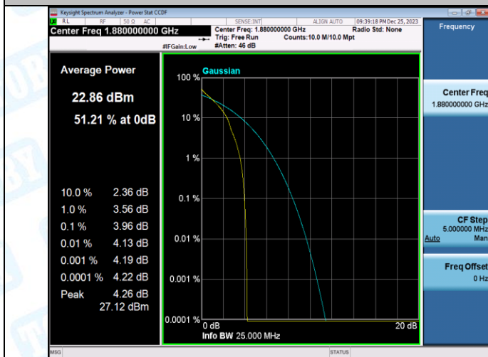
Band2-15MHz-QPSK-18900-75RB#0-PASS
