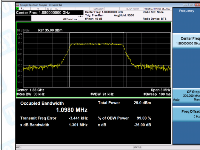
Band2-1.4MHz-16QAM-19193-6RB#0-PASS
