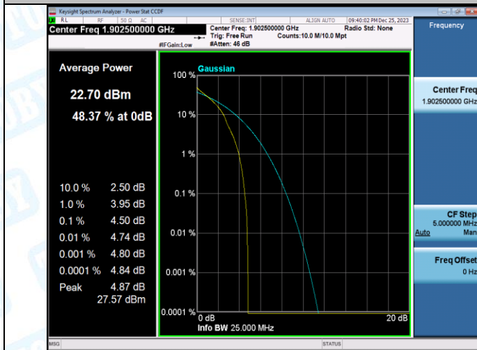
Band2-15MHz-QPSK-19125-75RB#0-PASS
