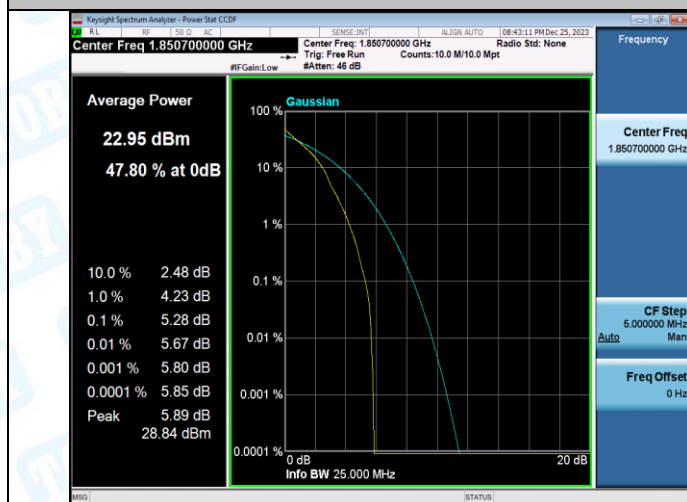
Band2-1.4MHz-QPSK-18607-6RB#0-PASS
