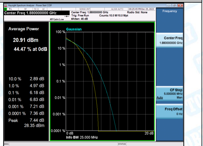
Band2-1.4MHz-16QAM-18607-1RB#0-PASS
