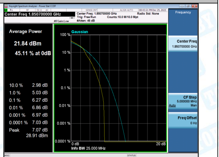
Band2-1.4MHz-16QAM-18607-6RB#0-PASS
