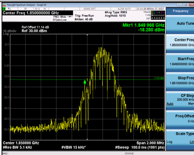
EGPRS1900-512-2-PASS
