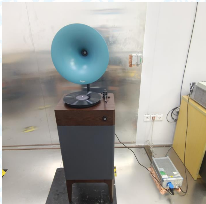
Photo of Setup for Conducted Emission
