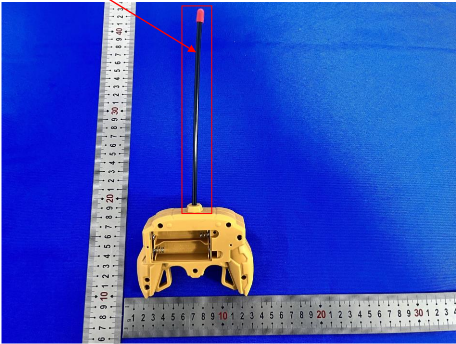
External Antenna
