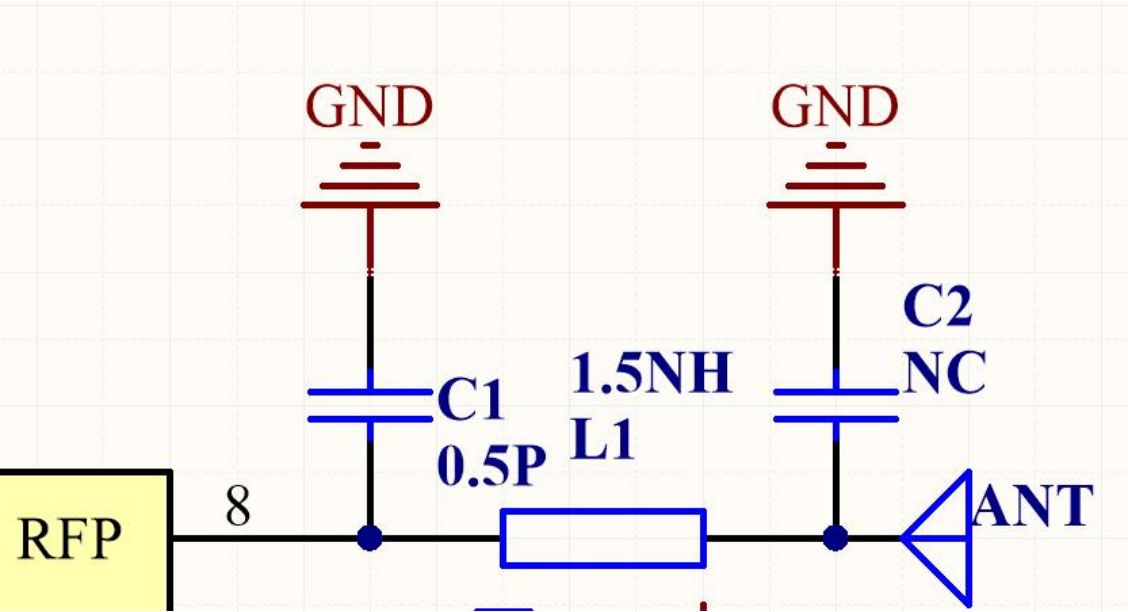
Match Network
