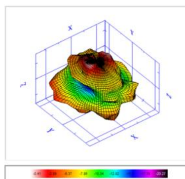
Radiation Pattern at 2500 MHz of Antenna.
