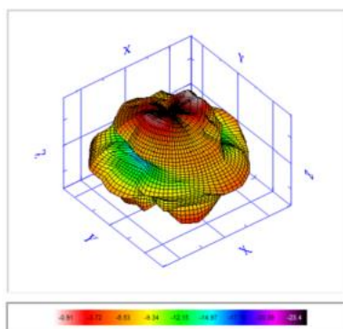
Radiation Pattern at 2480 MHz of Antenna.
