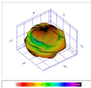
Radiation Pattern at 2400 MHz of Antenna.
