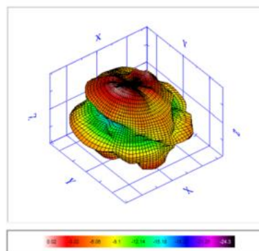
Radiation Pattern at 2450 MHz of Antenna.
