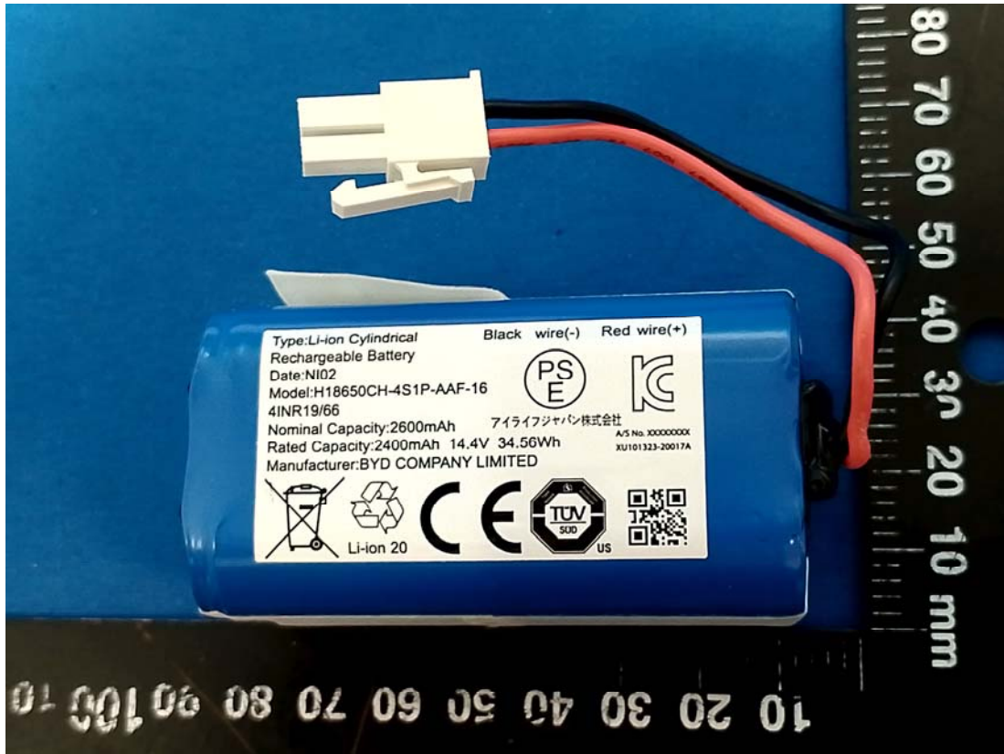
Battery 2#
