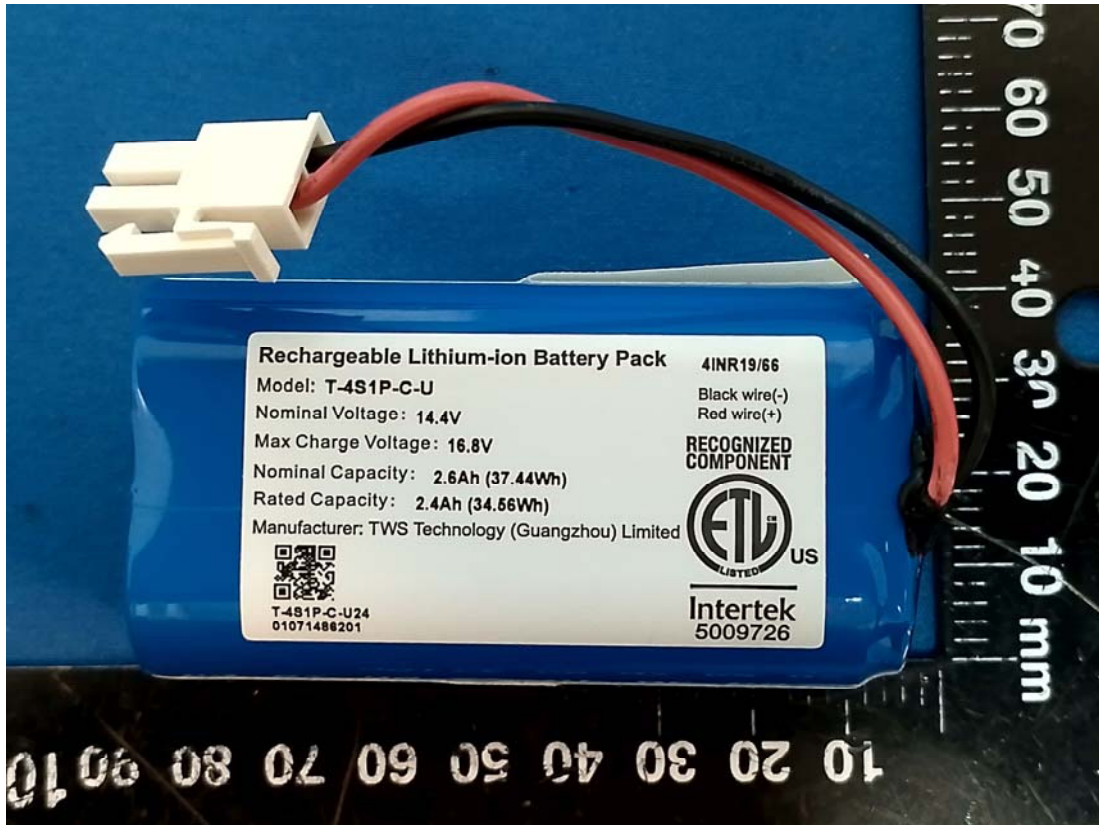
Battery 1#
