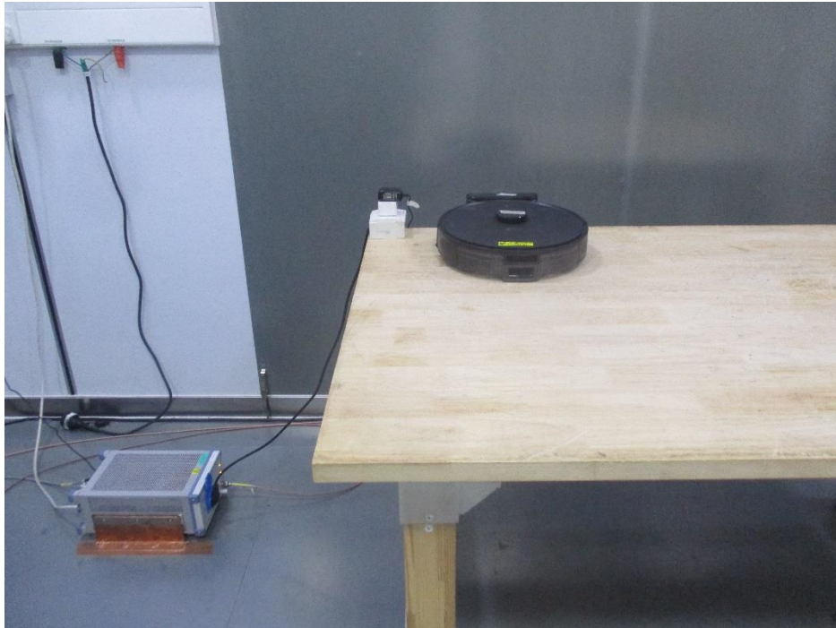
Radiated emission
