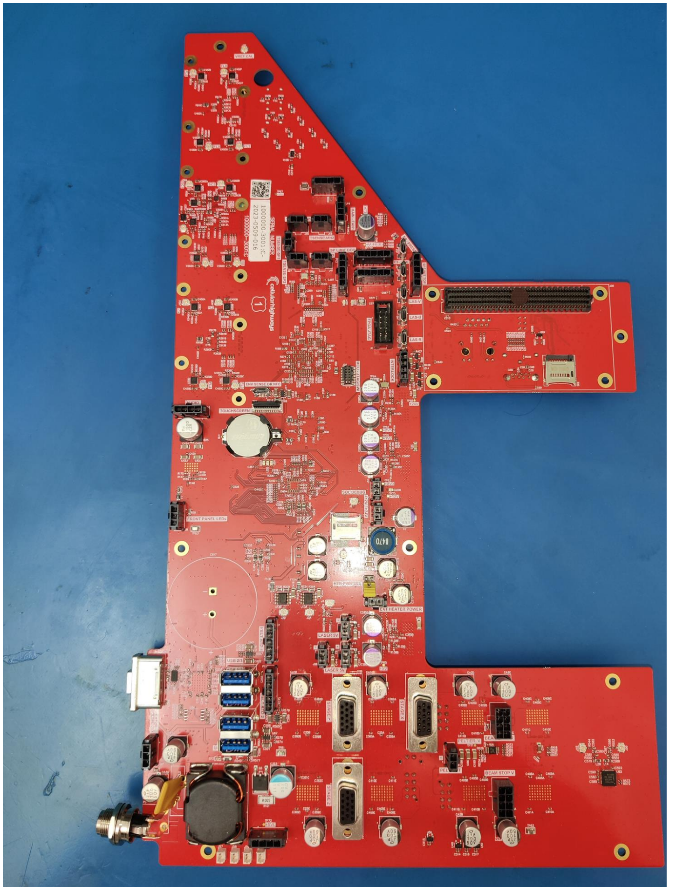
10000-1001 Highway1 main PCB front view
