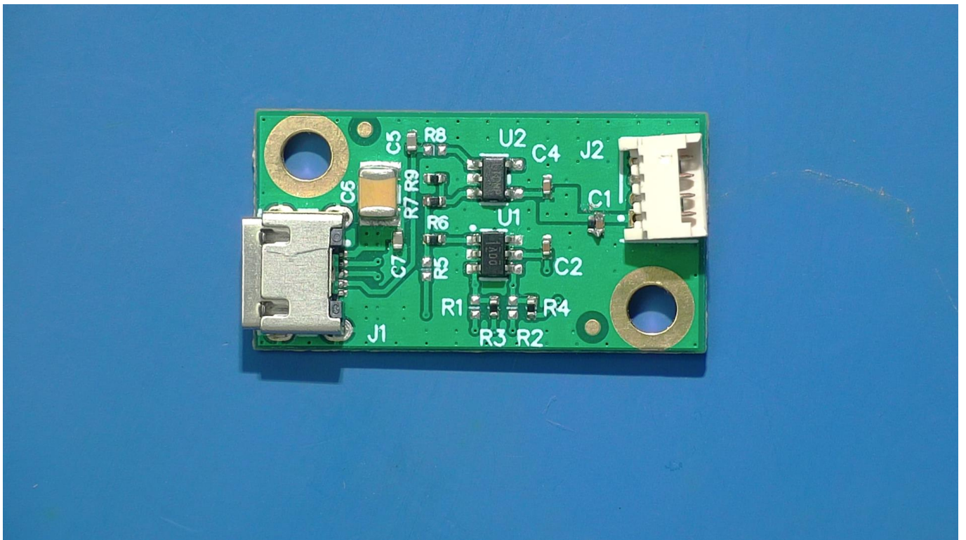
10000-1001 Highway1 load cell interface PCB front view
