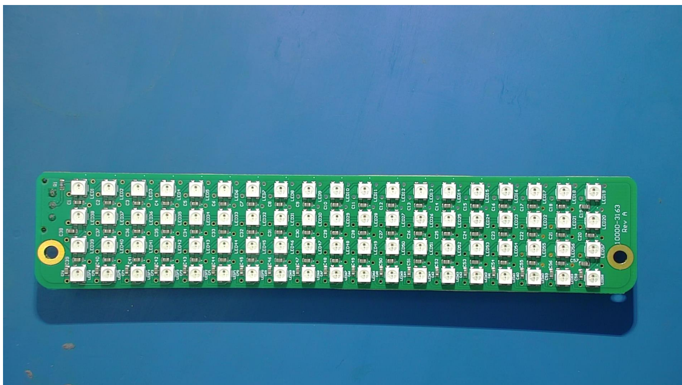
10000-1001 Highway1 display LED PCB front view
