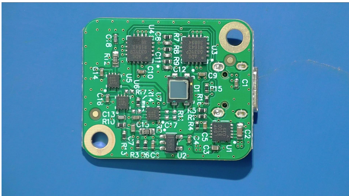
10000-1001 Highway1 Photodiode PCB front view
