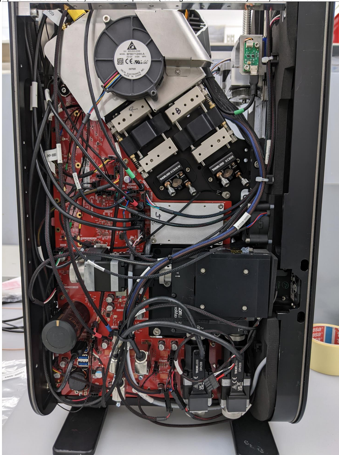
10000-1001 Highway1 (serial 4500000021) left internal view
