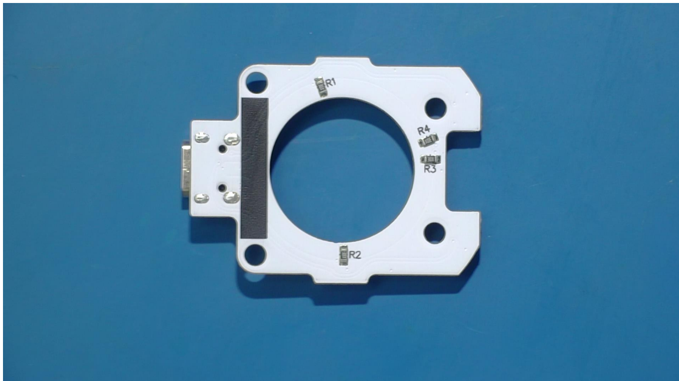
10000-1001 Highway1 heater interface & ringlight PCB back view
