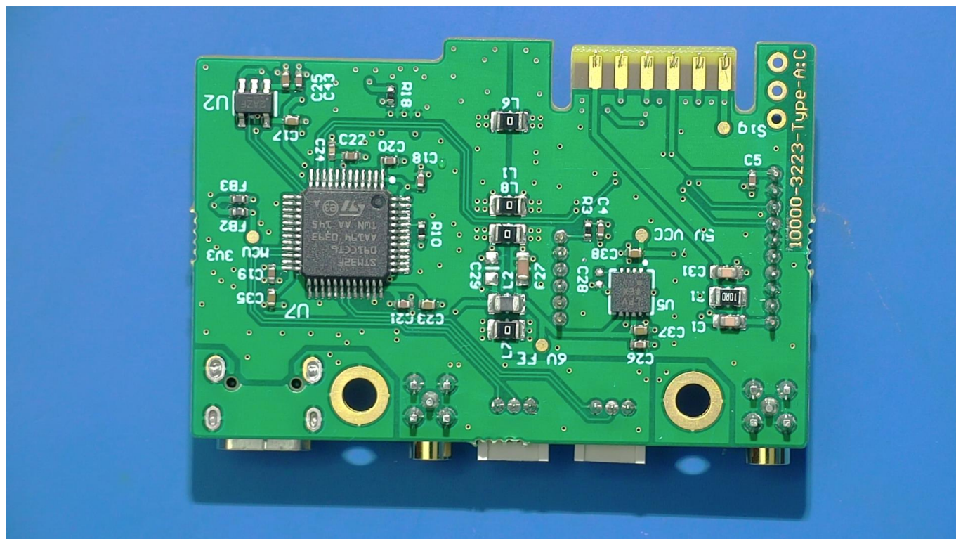
10000-1001 Highway1 Silicon Photomultiplier PCB back view
