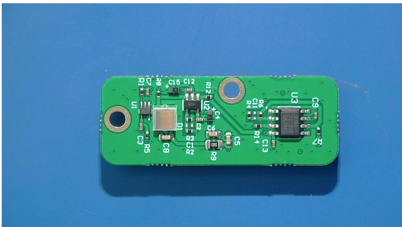
10000-1001 Highway1 Silicon Photomultiplier daughter PCB front view
