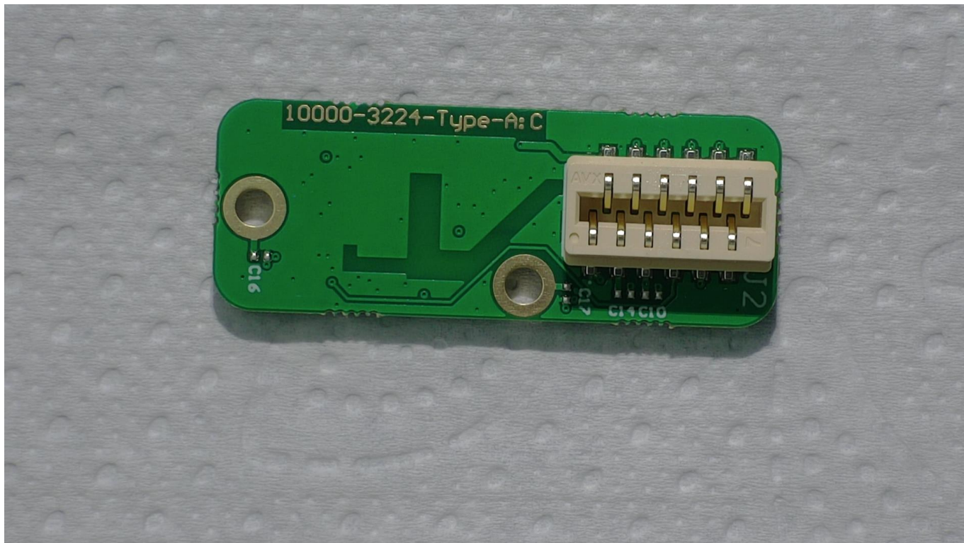
10000-1001 Highway1 Silicon Photomultiplier daughter PCB back view
