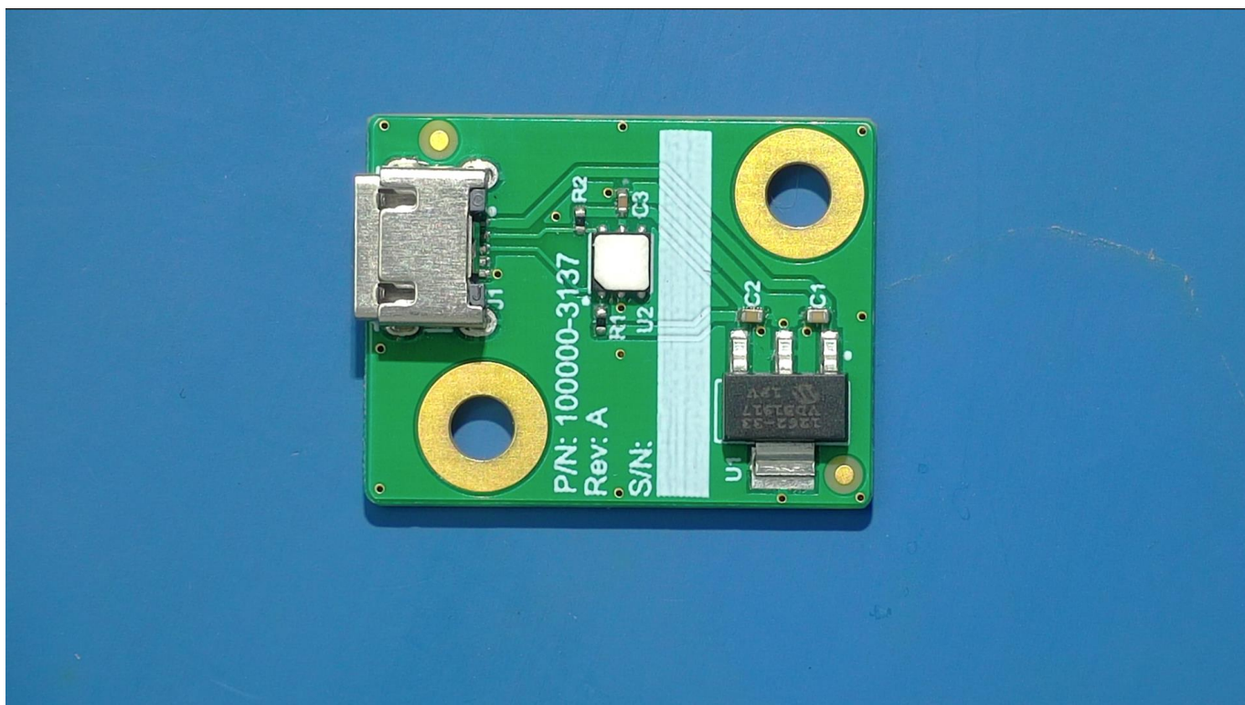
10000-1001 Highway1 environmental sensor PCB front view
