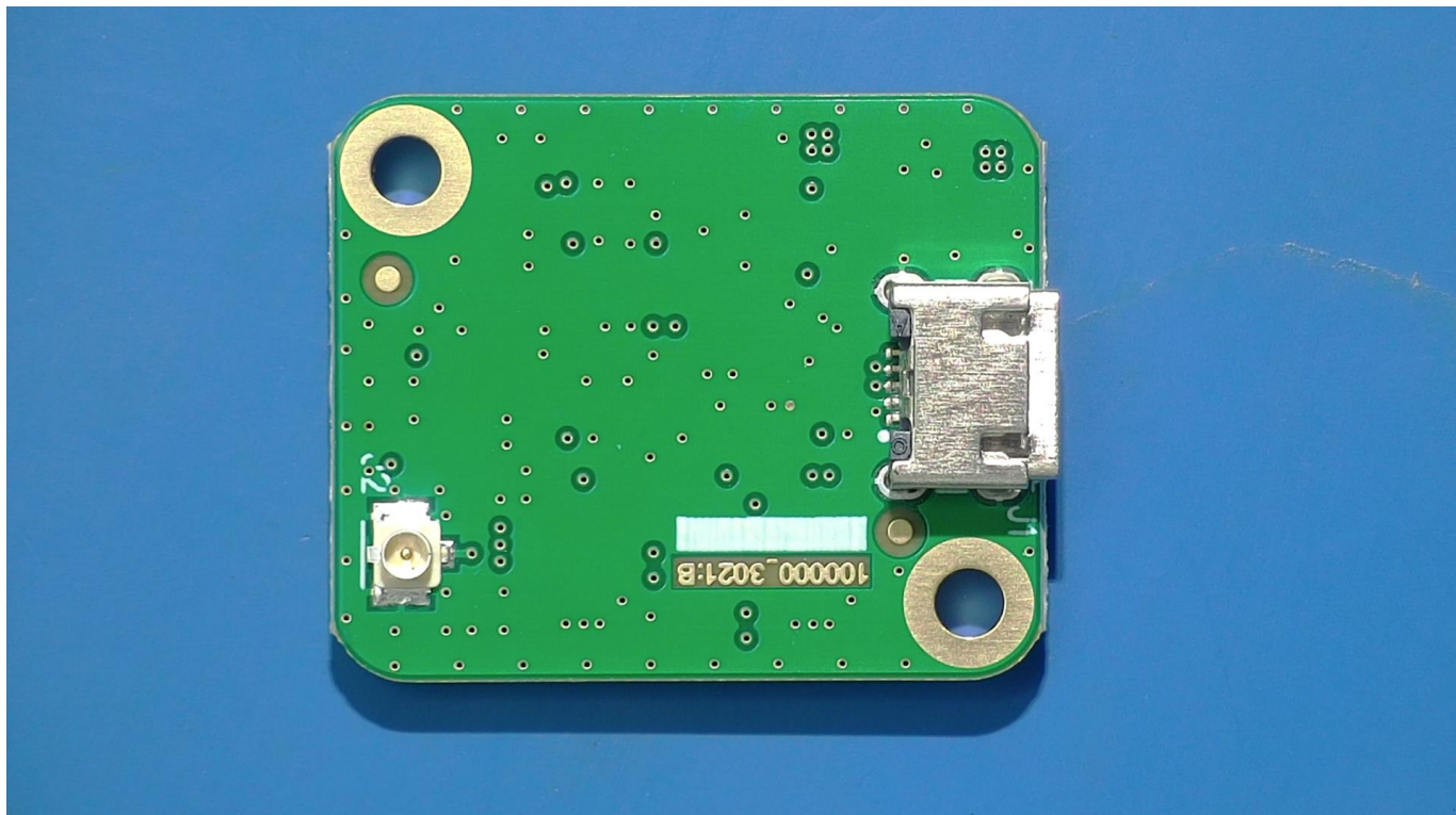
10000-1001 Highway1 Photodiode PCB back view
