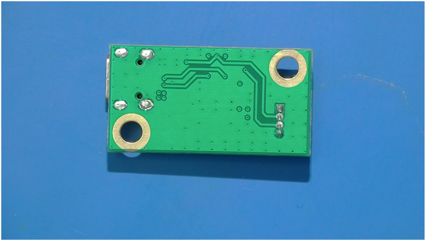
10000-1001 Highway1 load cell interface PCB back view
