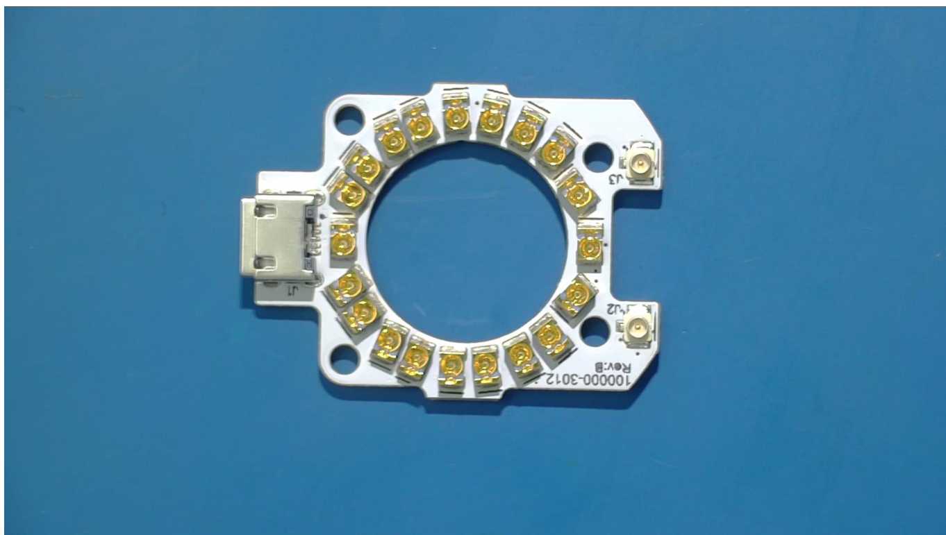
10000-1001 Highway1 heater interface & ringlight PCB front view
