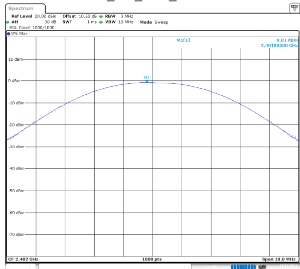
BLE_1M_Low_Channel
