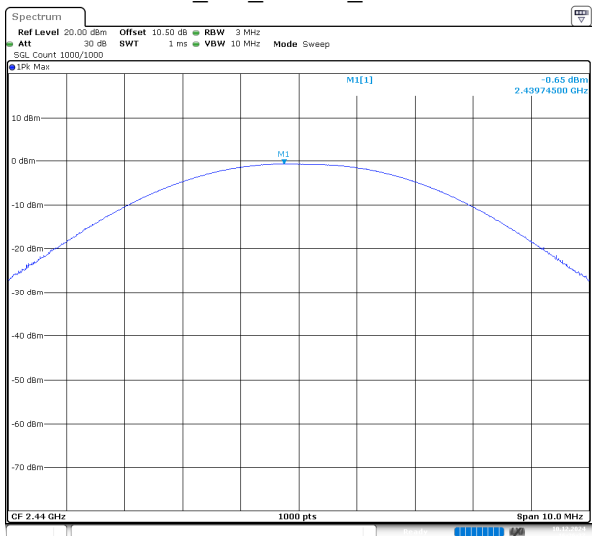
BLE_1M_Middle_Channel
