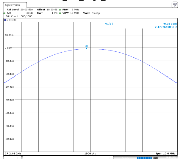
BLE_1M_High_Channel
