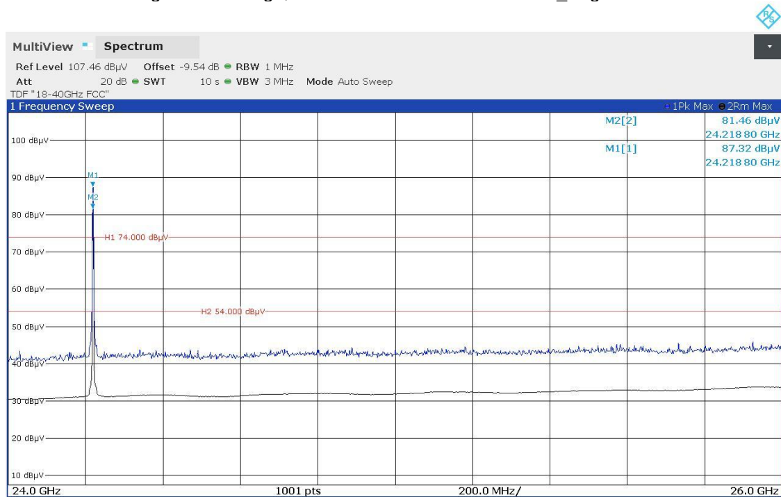
Plots No. 19: Radiated Higher Band-edge, Horizontal / Vertical Polarization _ High Channel
