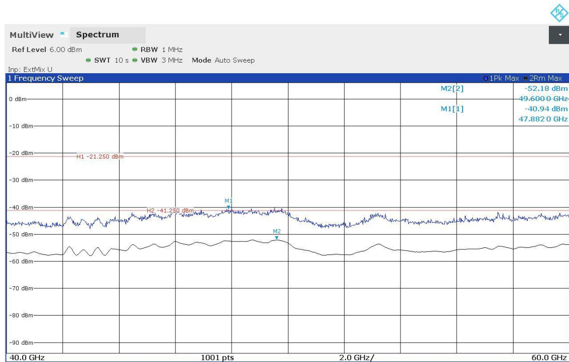
Plots No. 14: 40 GHz to 60 GHz, Horizontal / Vertical Polarization _ Low Channel
