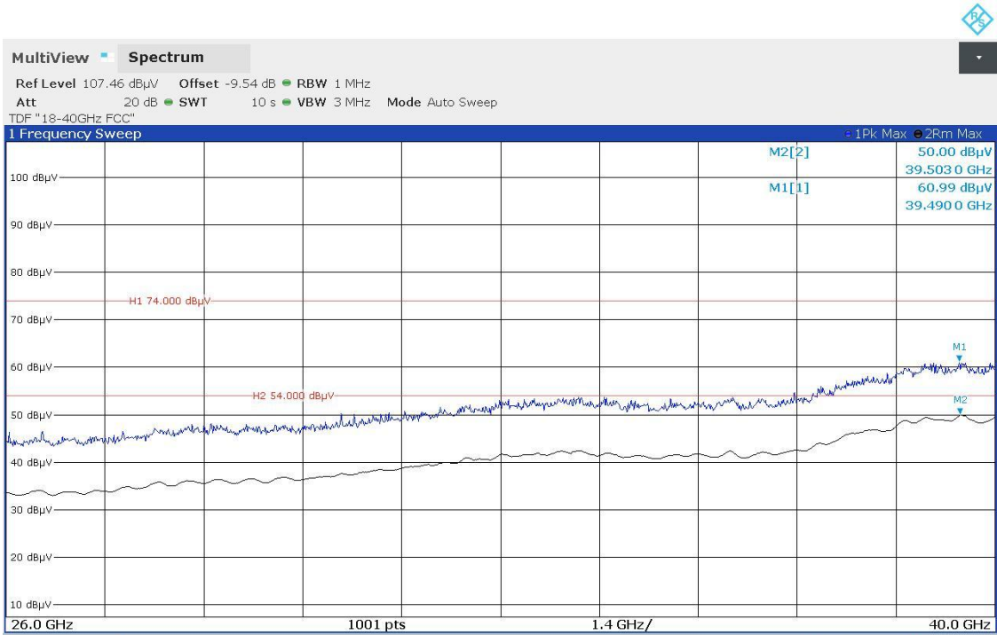
Plots No. 13: 26 GHz to 40 GHz, Horizontal / Vertical Polarization _ Middle Channel
