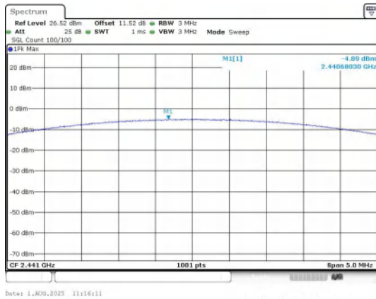
Peak Output Power \pi /4QPSK_Channel 39
