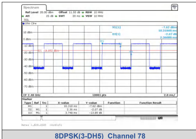
8DPSK(3-DH5)_Channel 78
