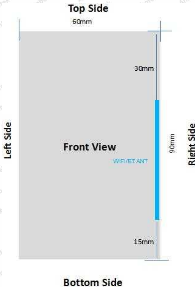
Distance of The Antenna to the EUT surface and edge
