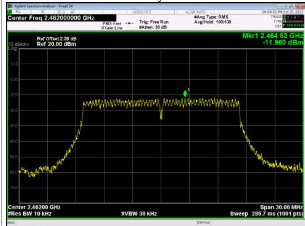
PSD NVNT g 2462MHz
