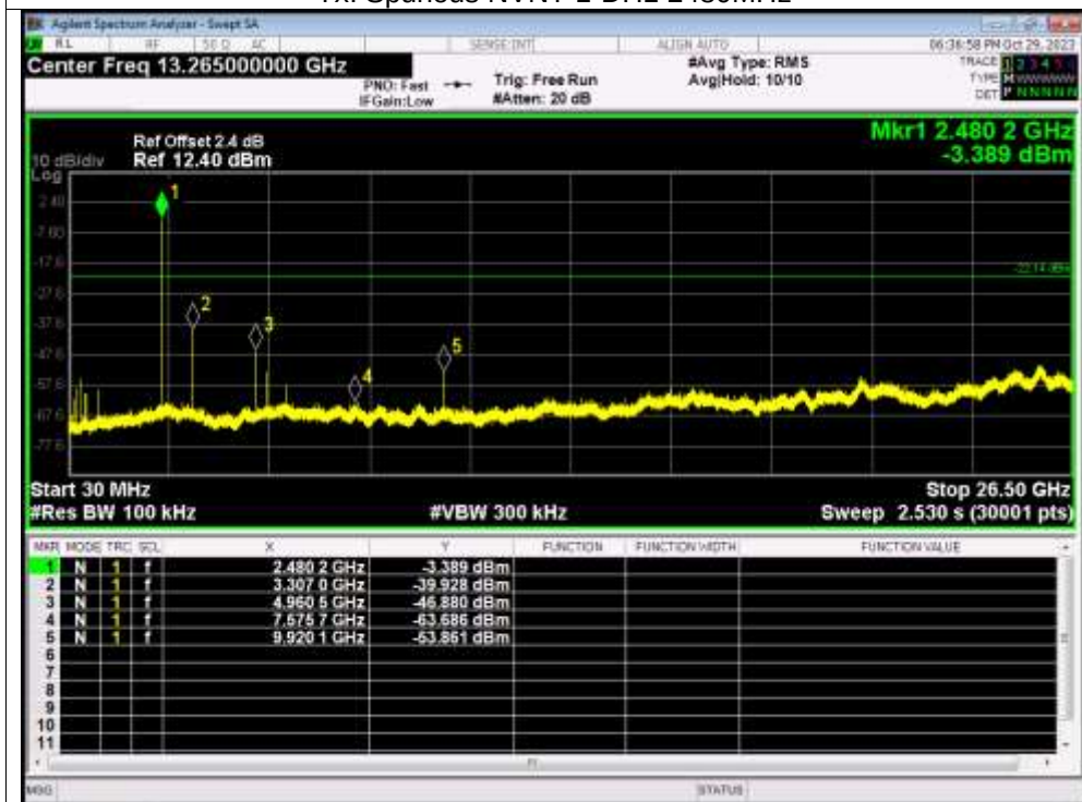
Tx. Spurious NVNT 1-DH1 2480MHz
