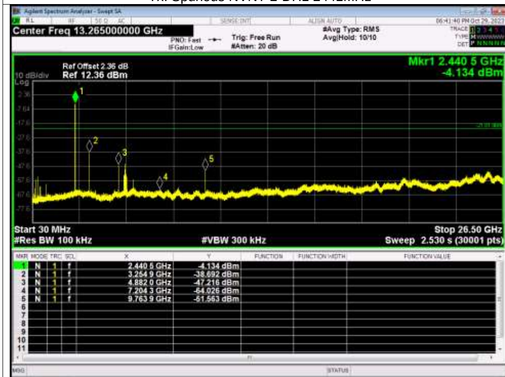
Tx. Spurious NVNT 2-DH1 2441MHz
