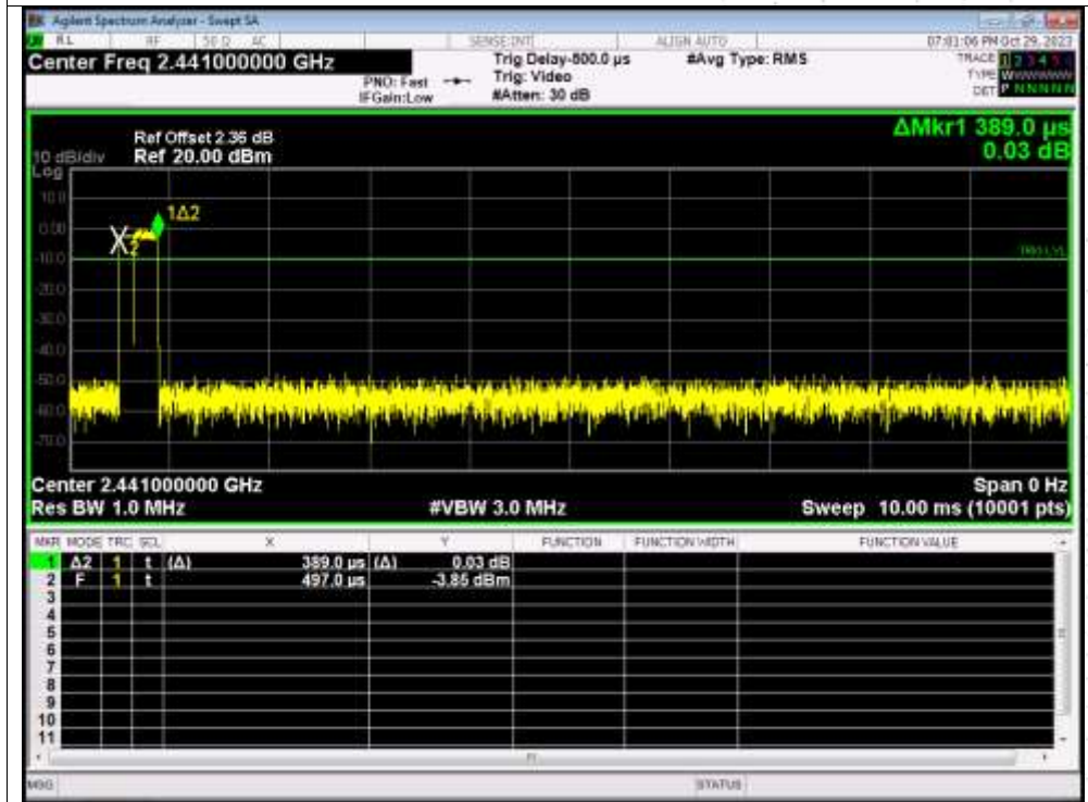
Dwell NVNT 3-DH3 2441MHz One Burst
