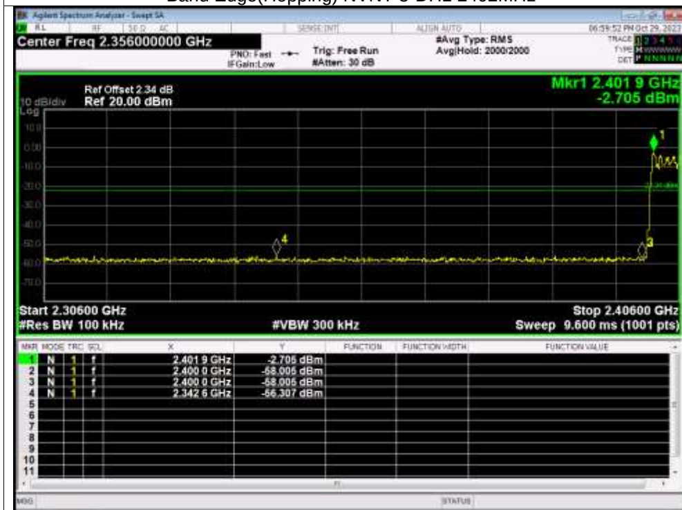
Band Edge(Hopping) NVNT 3-DH1 2402MHz
