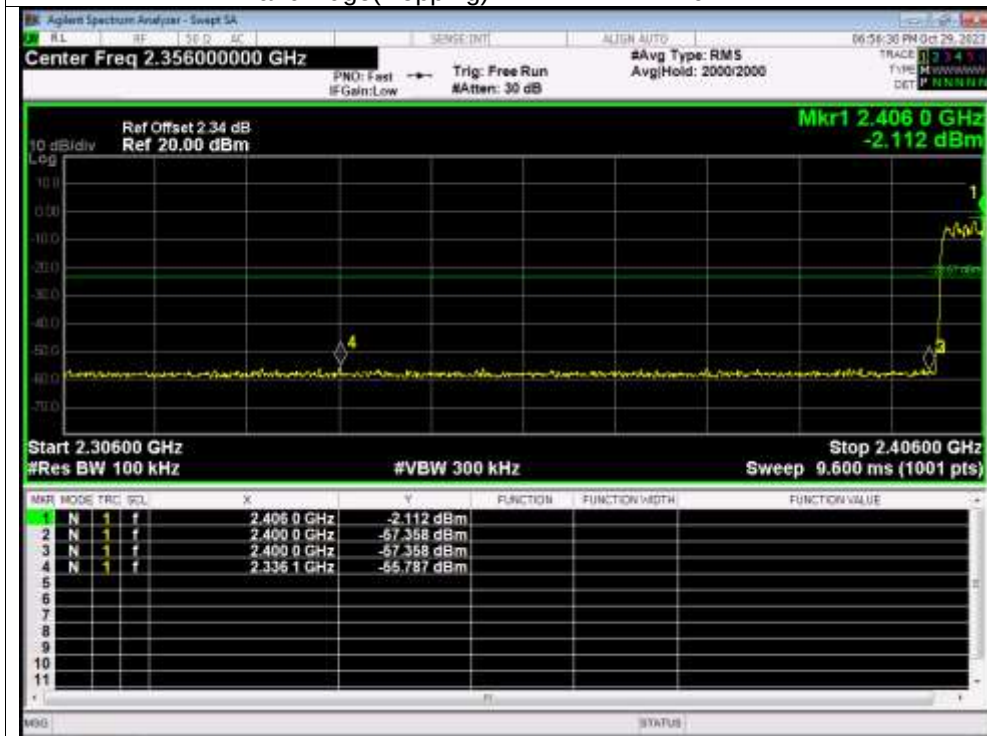
Band Edge(Hopping) NVNT 2-DH1 2402MHz
