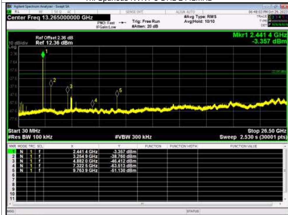
Tx. Spurious NVNT 3-DH1 2441MHz
