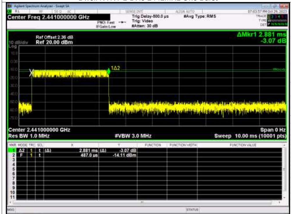
Dwell NVNT 2-DH1 2441MHz One Burst
