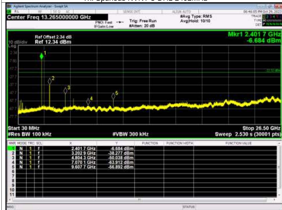
Tx. Spurious NVNT 3-DH1 2402MHz
