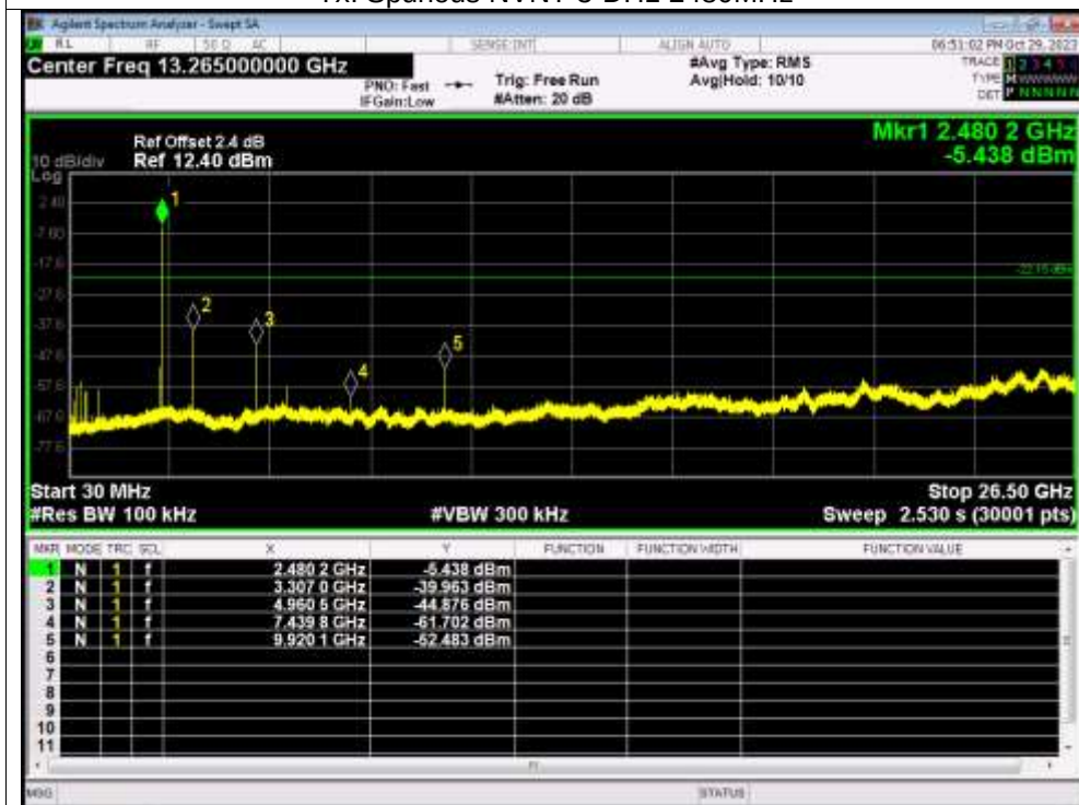
Tx. Spurious NVNT 3-DH1 2480MHz
