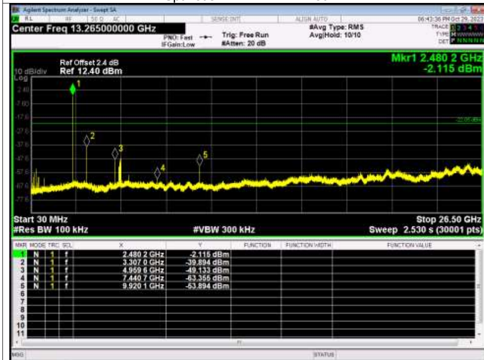
Tx. Spurious NVNT 2-DH1 2480MHz
