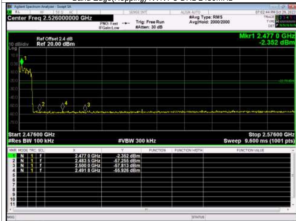
Band Edge(Hopping) NVNT 3-DH1 2480MHz
