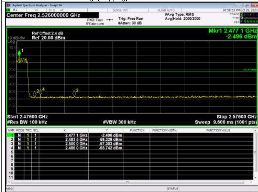
Band Edge(Hopping) NVNT 2-DH1 2480MHz
