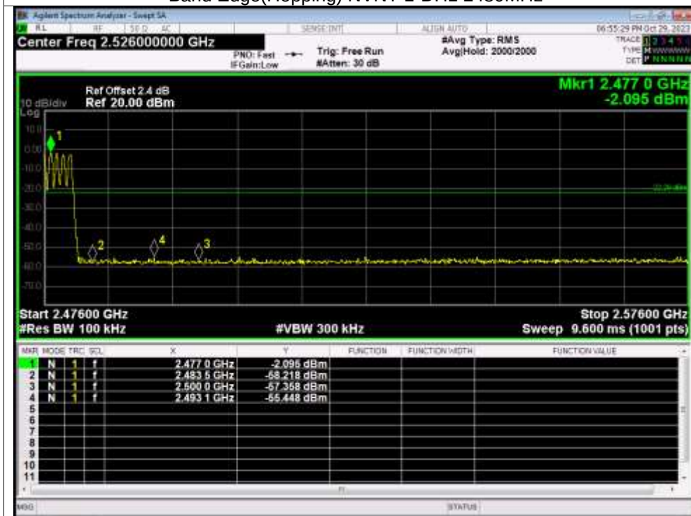
Band Edge(Hopping) NVNT 1-DH1 2480MHz
