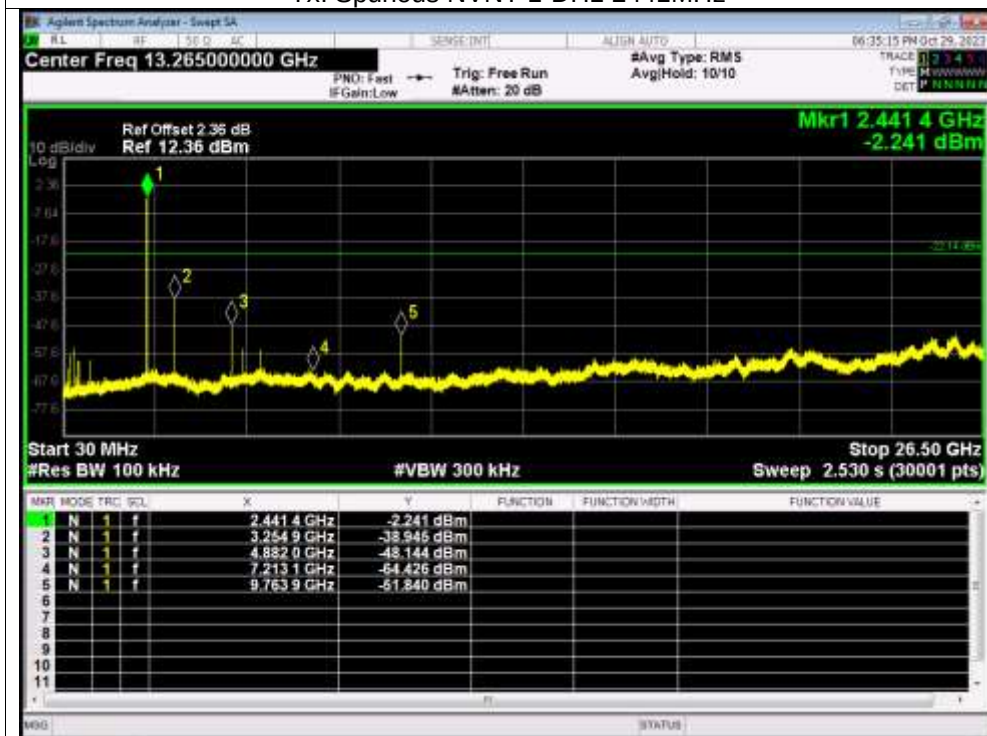
Tx. Spurious NVNT 1-DH1 2441MHz
