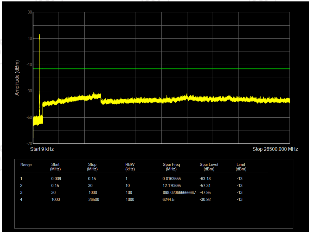
Band71 16QAM BW=5MHz Channel=133147 RB Size=25 Position=#0
