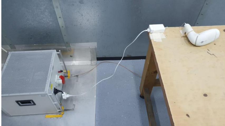
Picture 3 Conducted emission.
