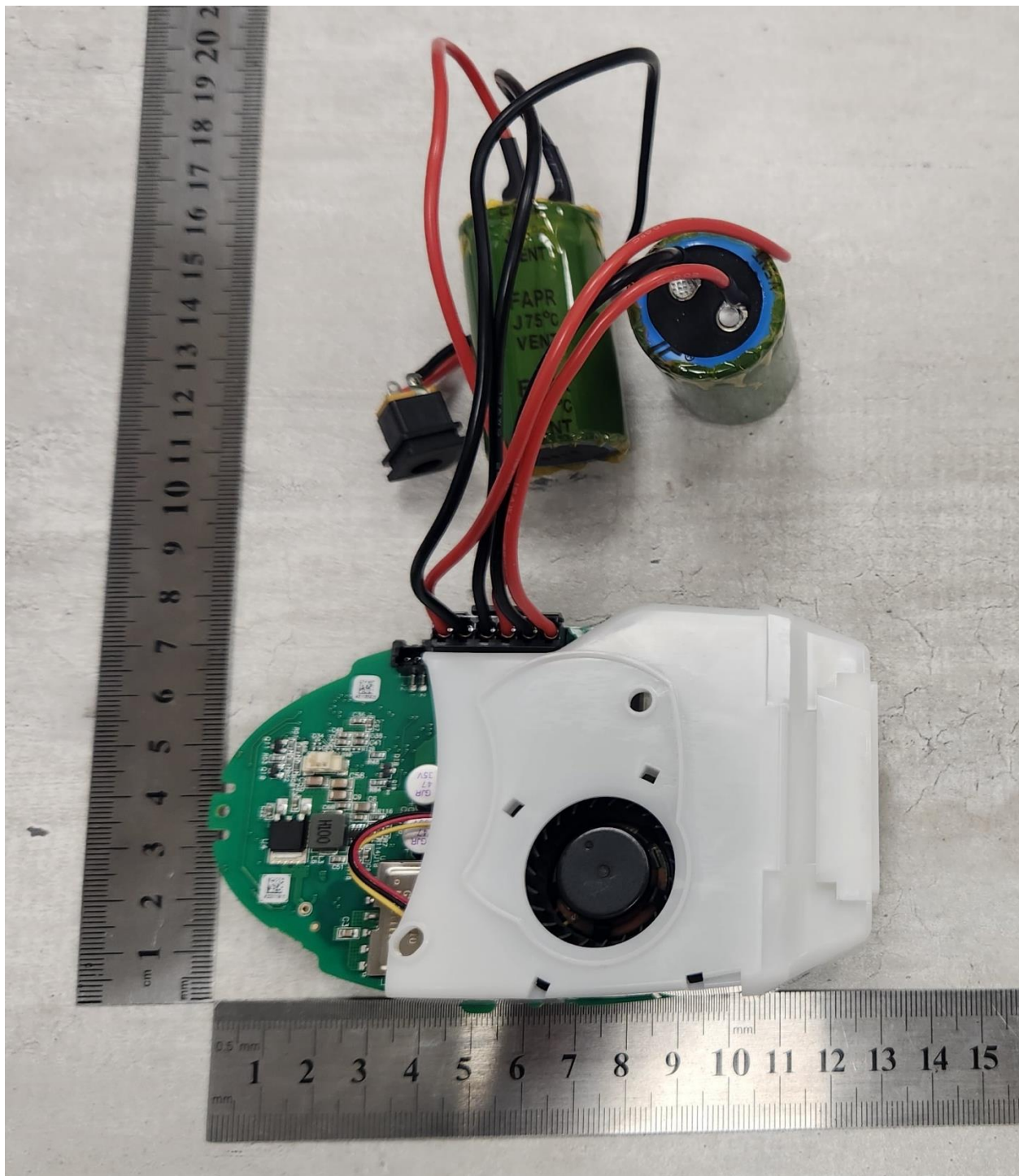
Bottom View
