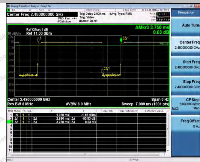
3DH5_Ant1_2480
