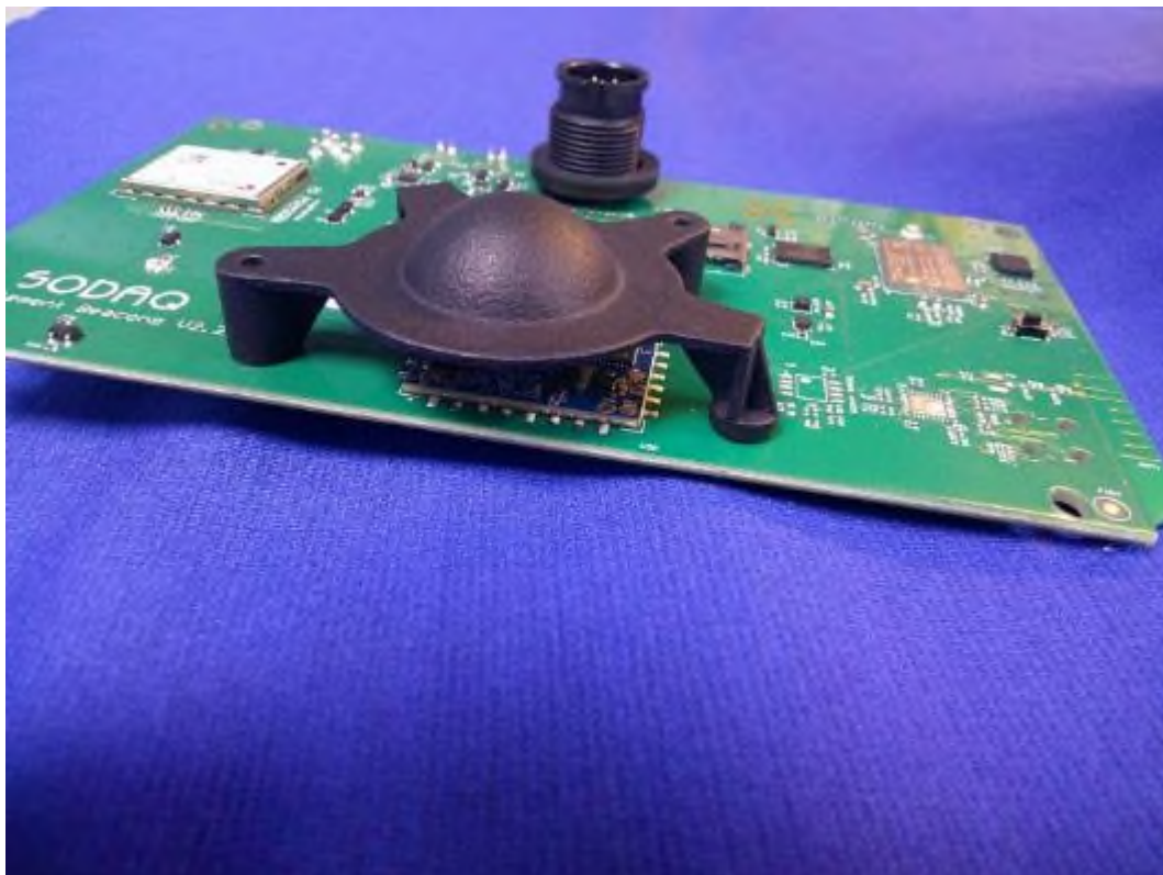
Photograph shows the EUTs 60 GHz RADAR antenna / lens
