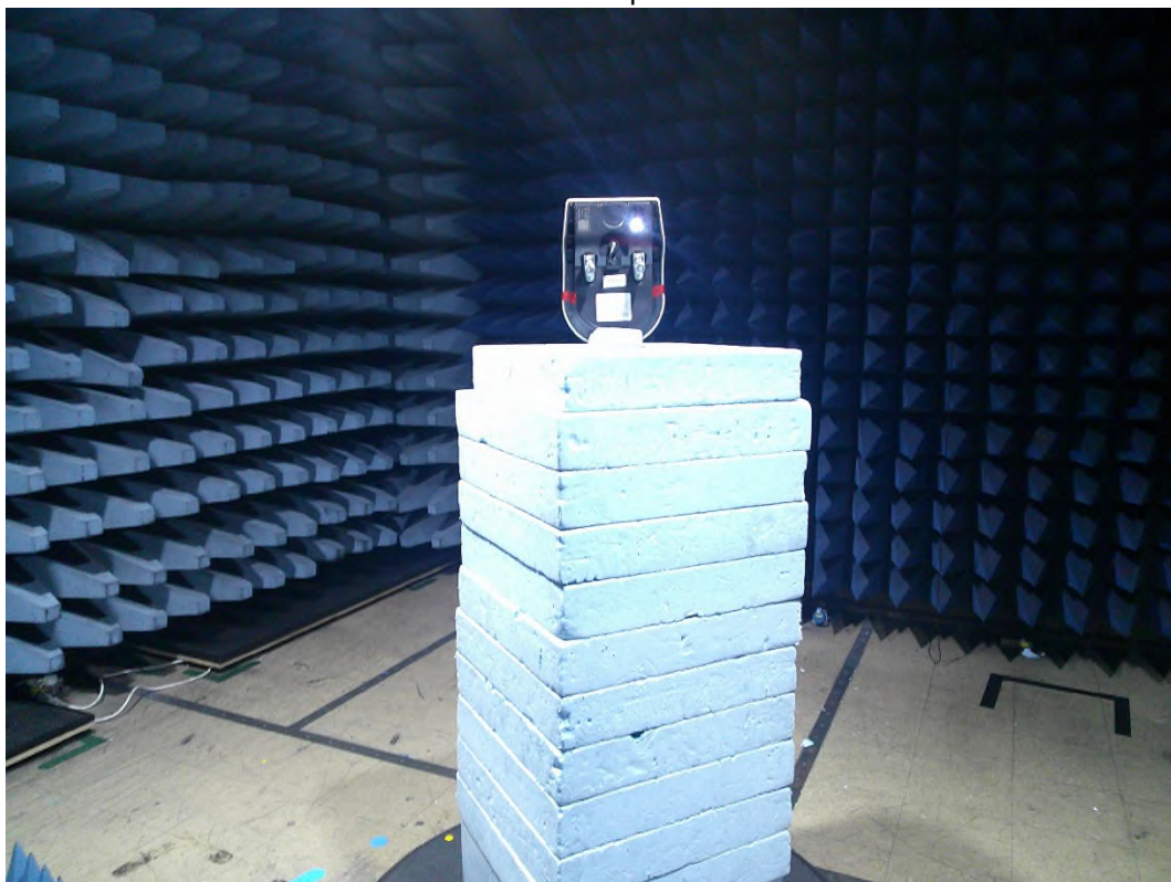
EUT in 'Upright' position
