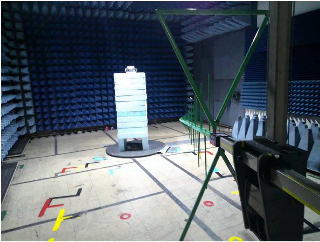
EUT in 'Flat' position
