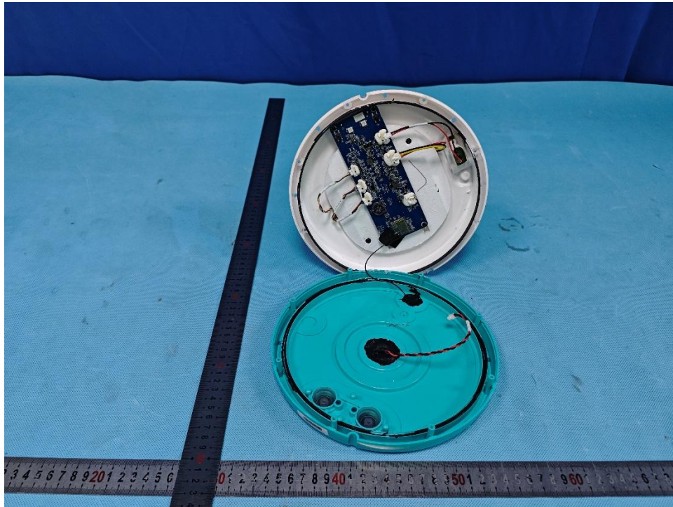
Internal photos(WTW2P)
