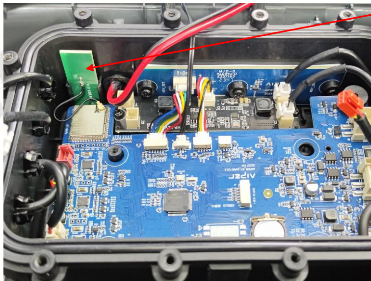
WiFi&BLE Antenna
