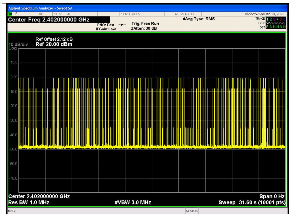
NVNT 3-DH5 2402MHz Ant One Burst
