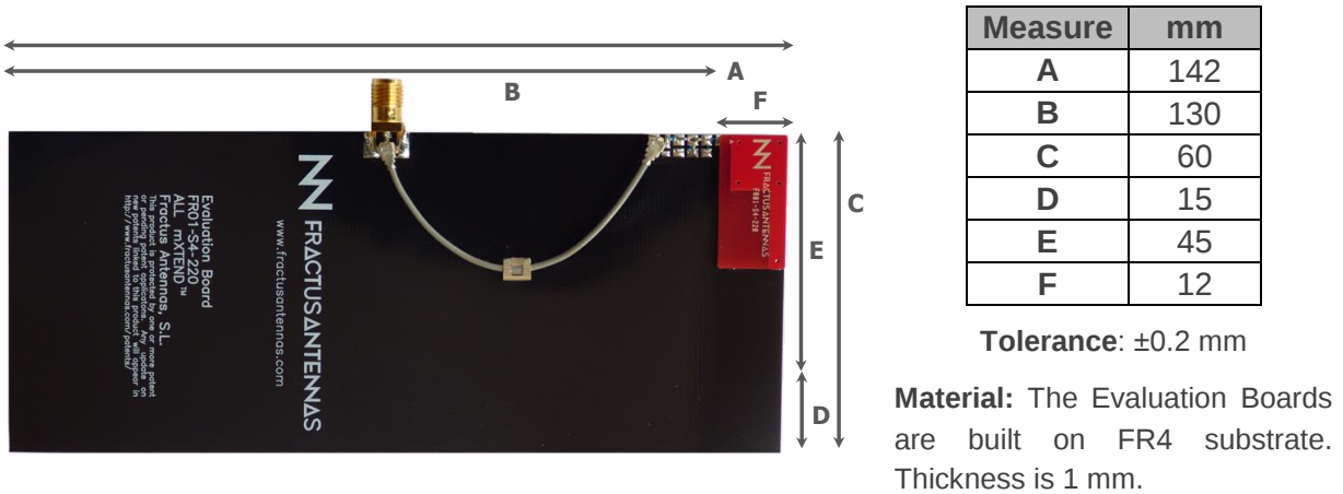
Figure 1 – EB_FR01-S4-220-1B-2R-1P. Evaluation Board 1 port providing operation in 2 frequency ranges, 698 – 960MHz and 1710 – 2690MHz.
