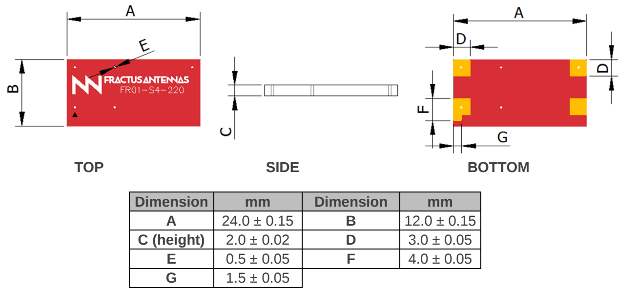
Figure 4 – ALL mXTEND™ chip antenna component dimensions and tolerances.
