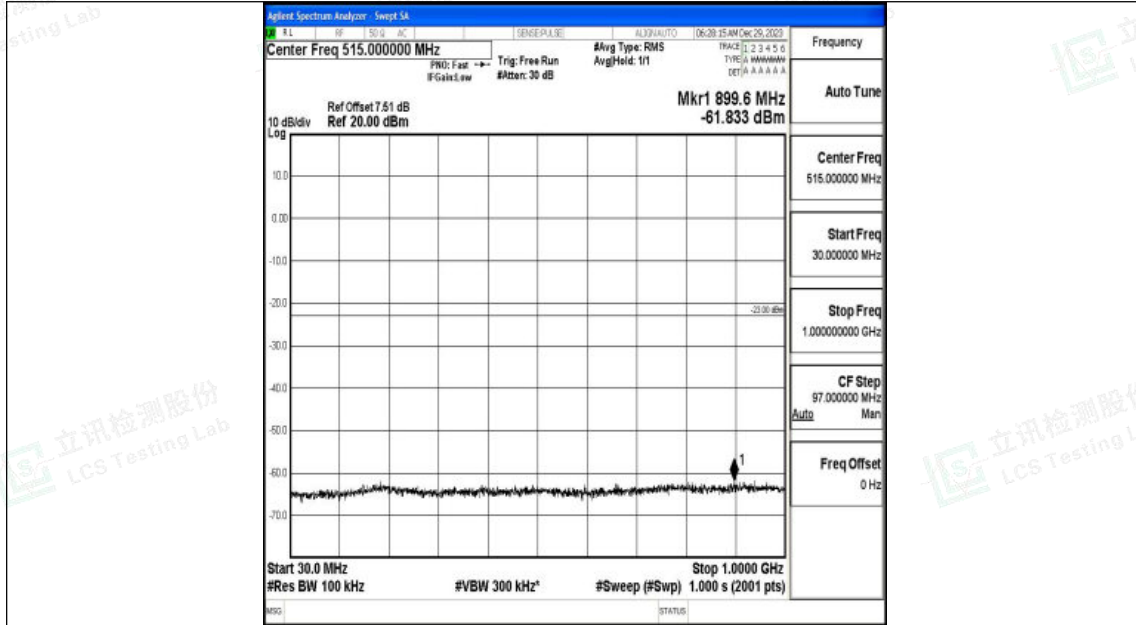
Band25_15MHz_QPSK_26365_1RB#0_30~1000_30~1000
