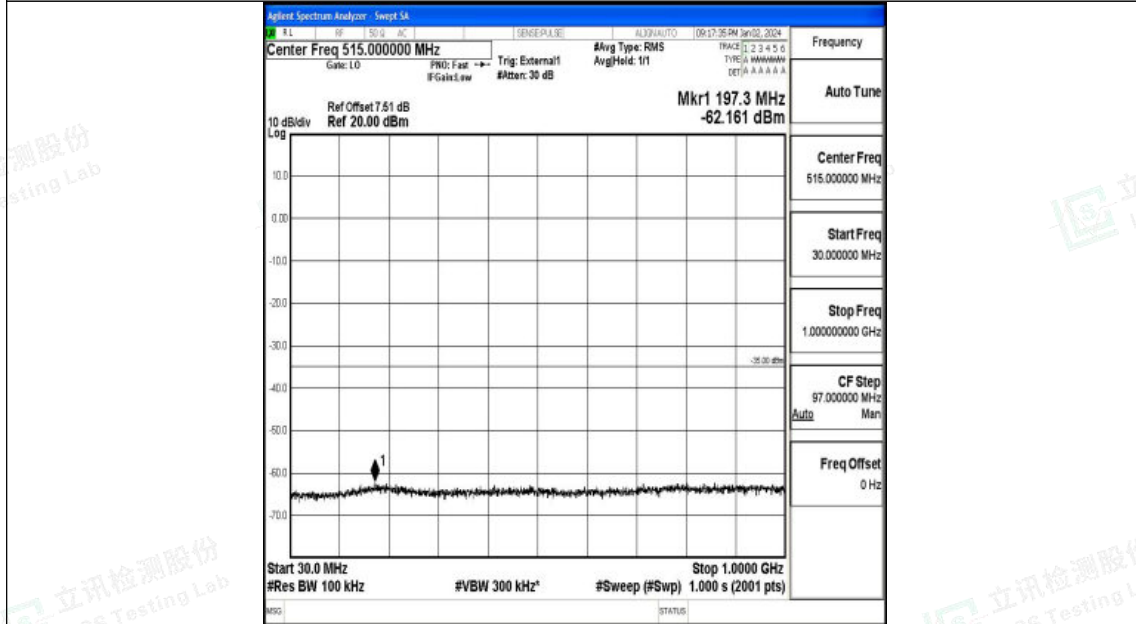
Band38_20MHz_16QAM_38150_1RB#0_30~1000_30~1000
