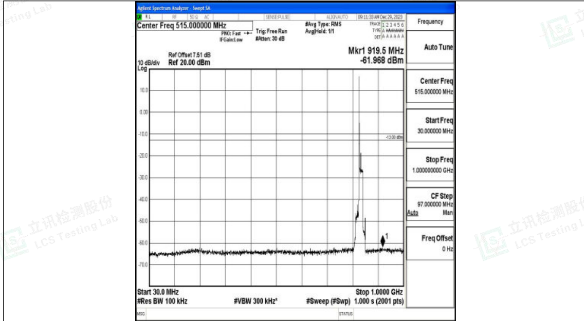
Band26_15MHz_QPSK_26915_1RB#0_30~1000_30~1000
