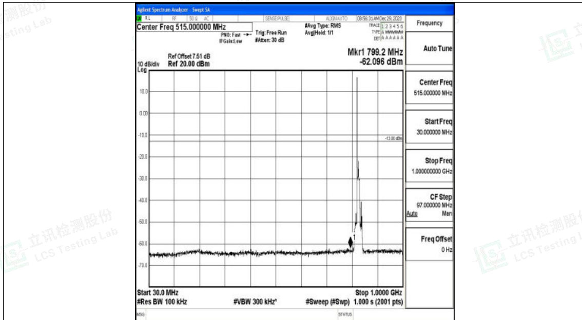
Band26_10MHz_QPSK_26840_1RB#0_30~1000_30~1000
