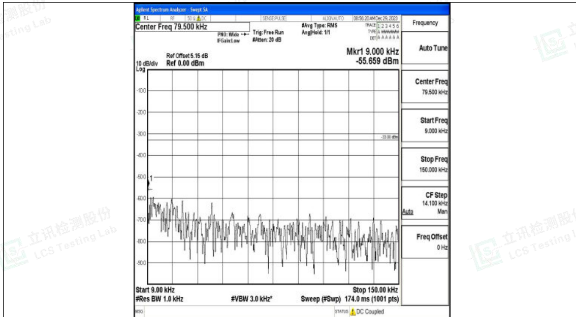
Band26_10MHz_QPSK_26840_1RB#0_0.009~0.15_0.009~0.15
