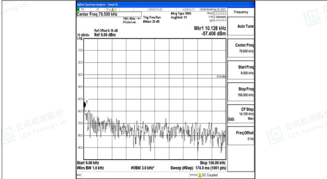
Band26_15MHz_QPSK_26865_1RB#0_0.009~0.15_0.009~0.15
