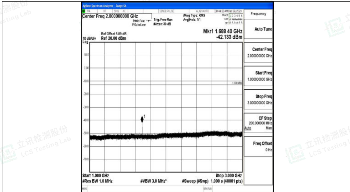
Band26_5MHz_16QAM_27015_1RB#0_1000~3000_1000~3000
