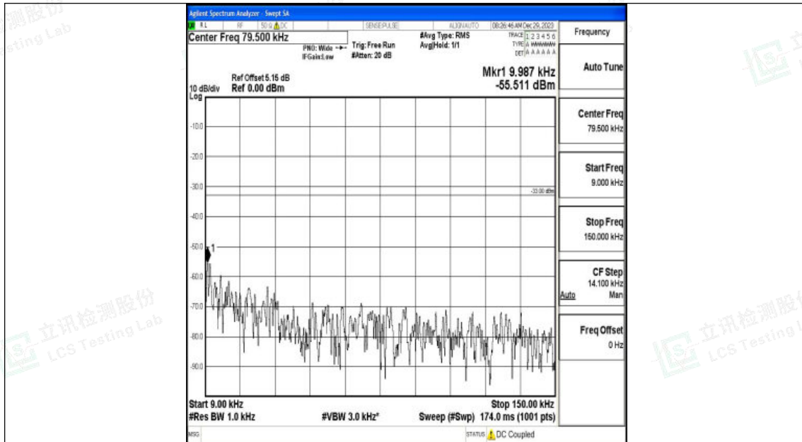
Band26_3MHz_QPSK_27025_1RB#0_0.009~0.15_0.009~0.15
