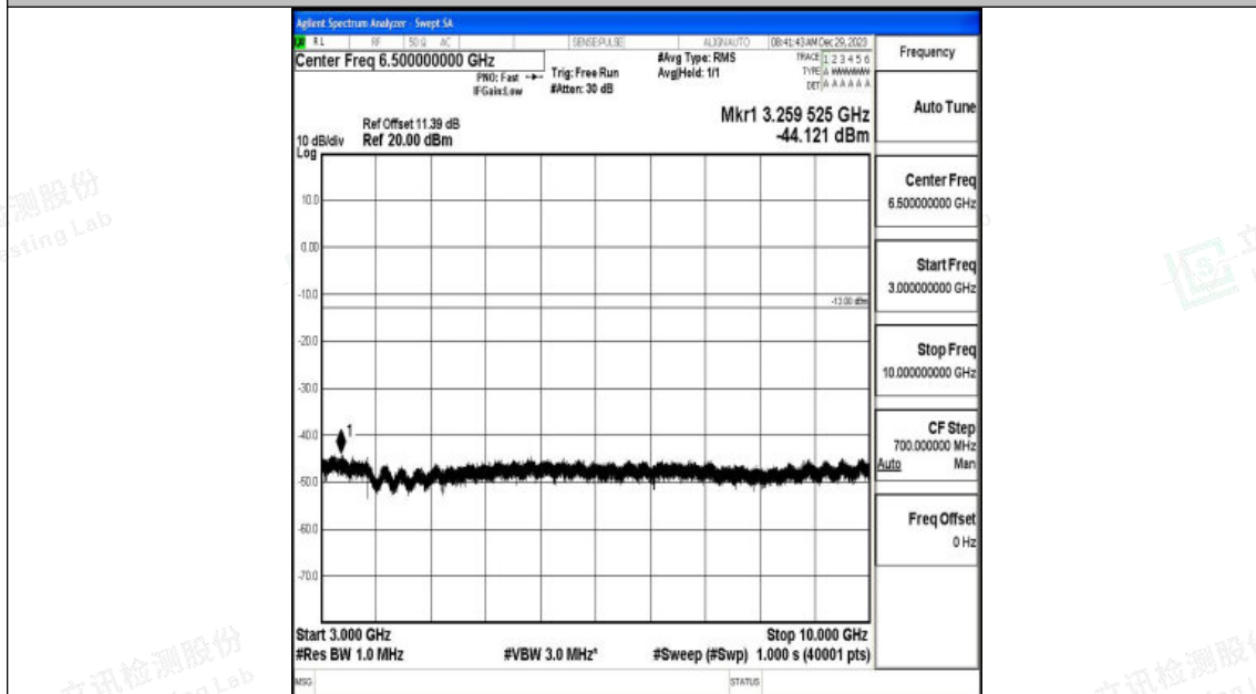
Band26_5MHz_16QAM_26815_1RB#0_3000~10000_3000~10000
