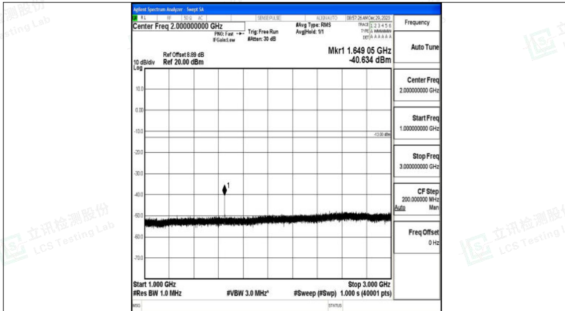
Band26_10MHz_16QAM_26840_1RB#0_1000~3000_1000~3000
