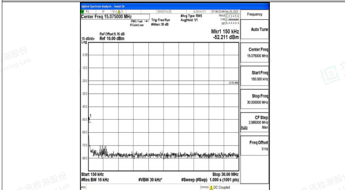
Band26_5MHz_QPSK_26765_1RB#0_0.15~30_0.15~30
