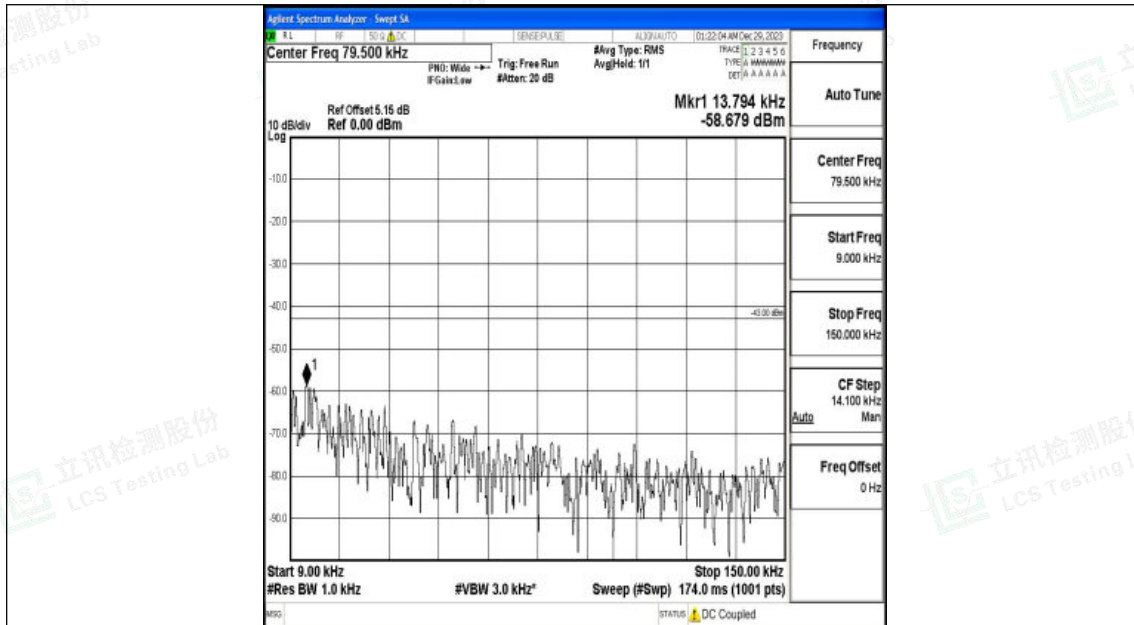
Band2_10MHz_QPSK_18650_1RB#0_0.009~0.15_0.009~0.15
