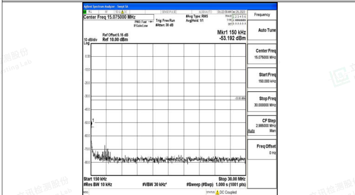
Band2_10MHz_QPSK_18650_1RB#0_0.15~30_0.15~30
