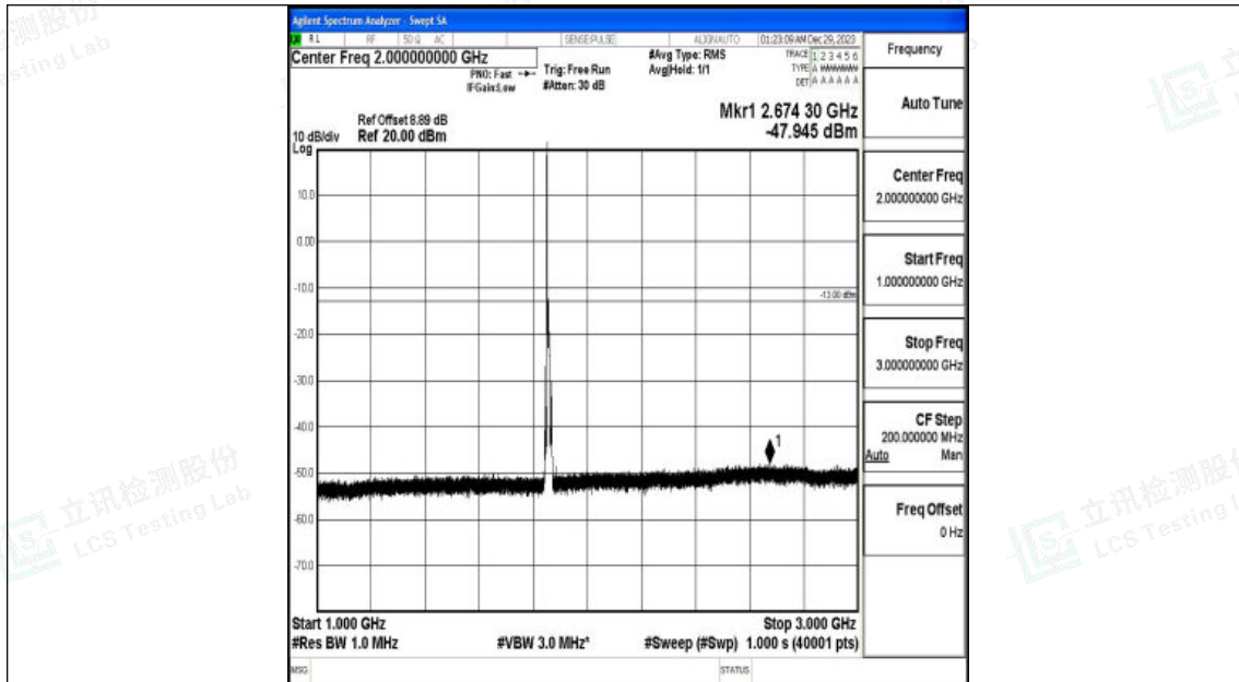
Band2_10MHz_16QAM_18650_1RB#0_1000~3000_1000~3000
