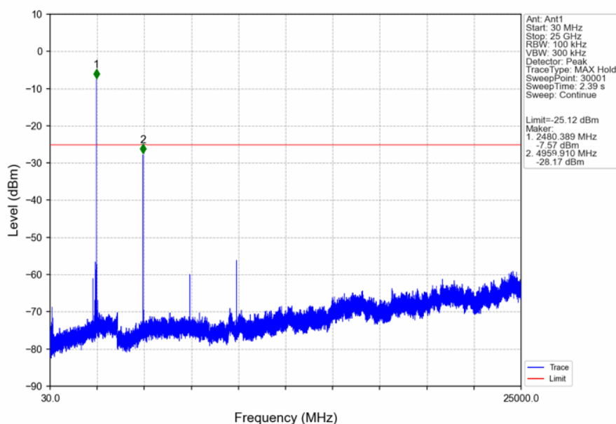
Pi/4DQPSK_2DH5_HCH_2480MHz_Ant1_NTNV
