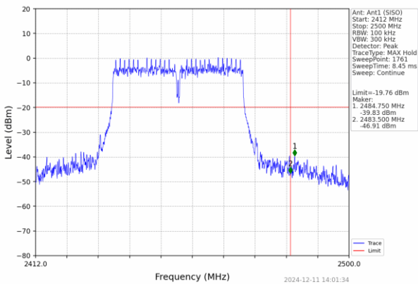
Right bandedge
