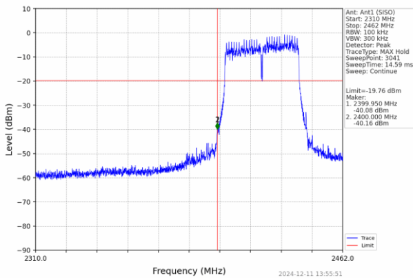
Left bandedge
