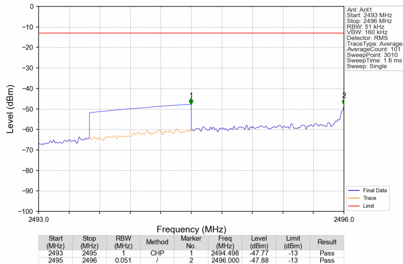
Band41_2498.5MHz_AWGN_SISO_Ant1_NTNV_AGC+3
