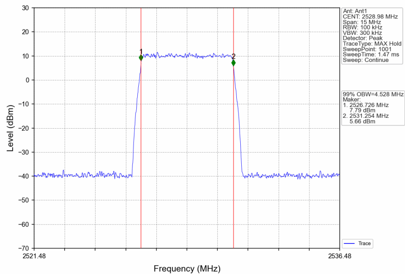
Band41_2528.98MHz_AWGN_SISO_Ant1_NTNV_Input_AGC+3
