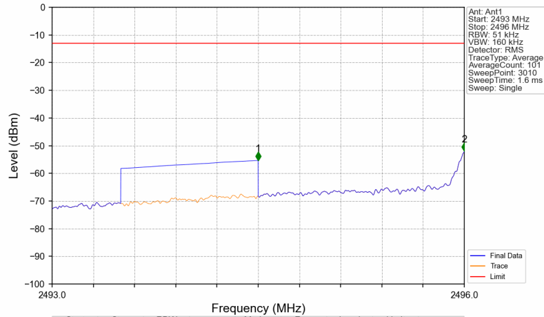
Band41_2498.5MHz_AWGN_SISO_Ant1_NTNV_AGC
