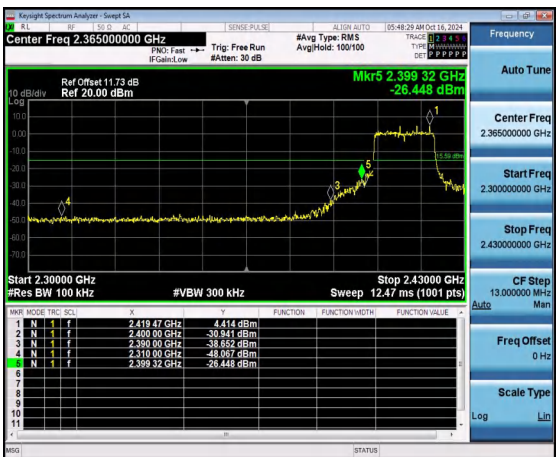
Left bandedge
