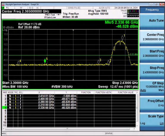
Left bandedge
