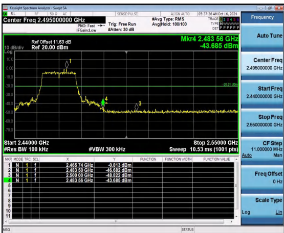
Right bandedge
