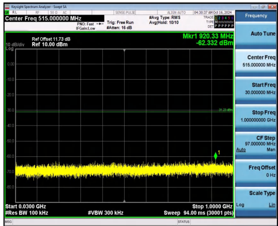
30MHz-1GHz
