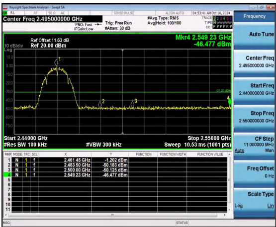
Right bandedge
