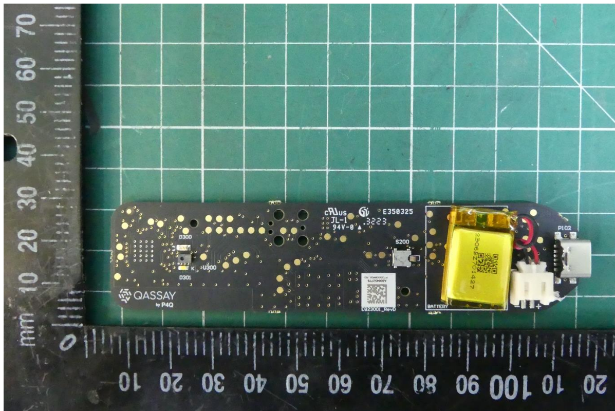
Bottom view PCB:
