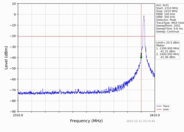
No-hopping mode
