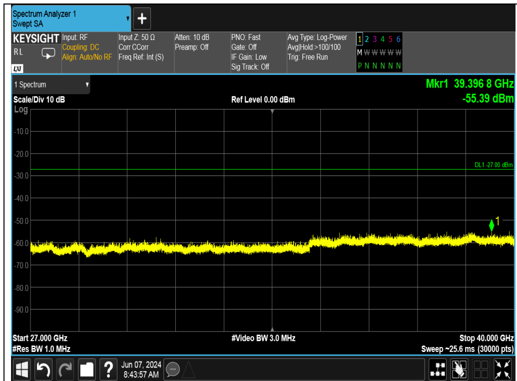
Test_Graph_802.11ac20_CHAIN A_5180_6Mbps_Frequency Band 5
