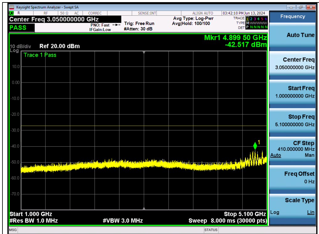
Test_Graph_802.11ac20_CHAIN B_5180_6Mbps_Frequency Band 2
