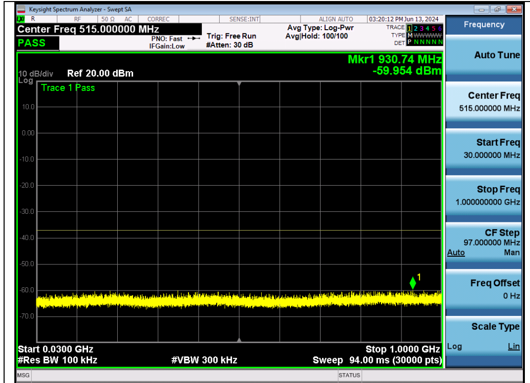
Test_Graph_802.11ac20_CHAIN A_5180_6Mbps_Frequency Band 1
