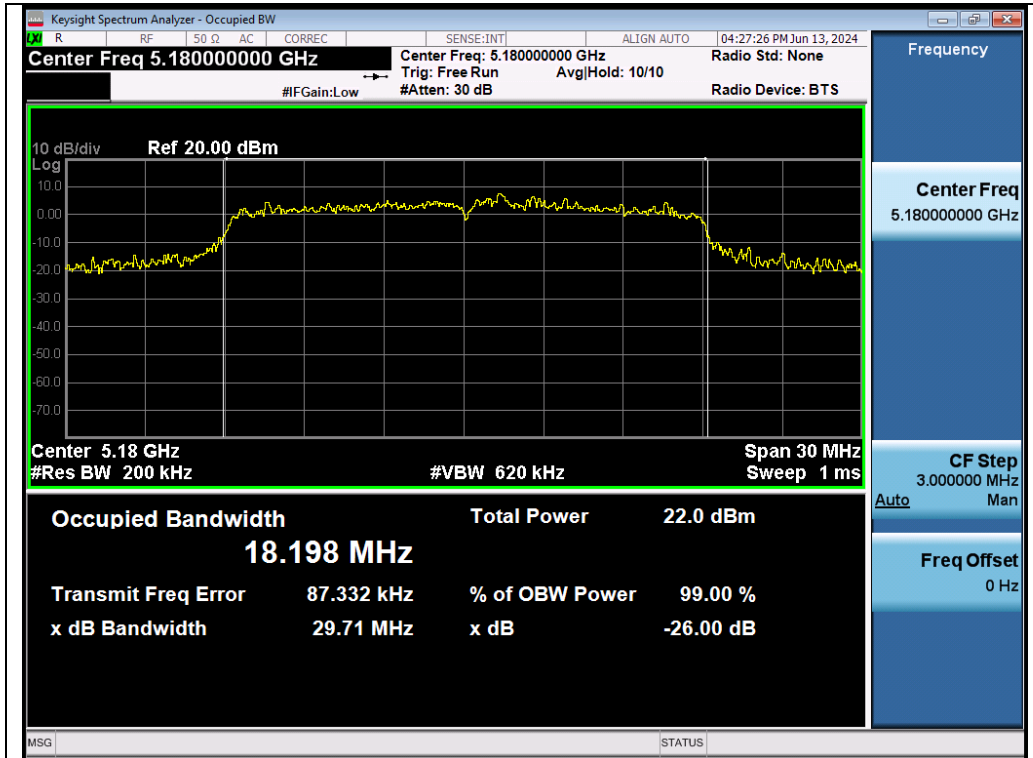
Test_Graph_802.11ac20_CHAIN A_5180_MCS0_OBW
