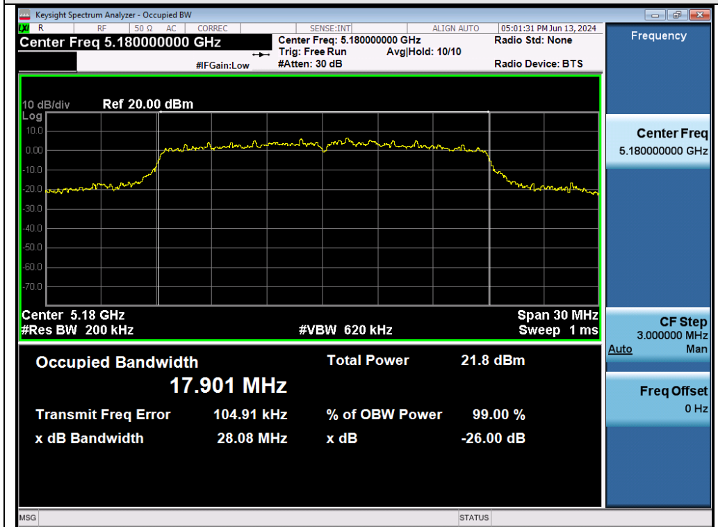
Test_Graph_802.11ac20_CHAIN B_5180_MCS0_OBW
