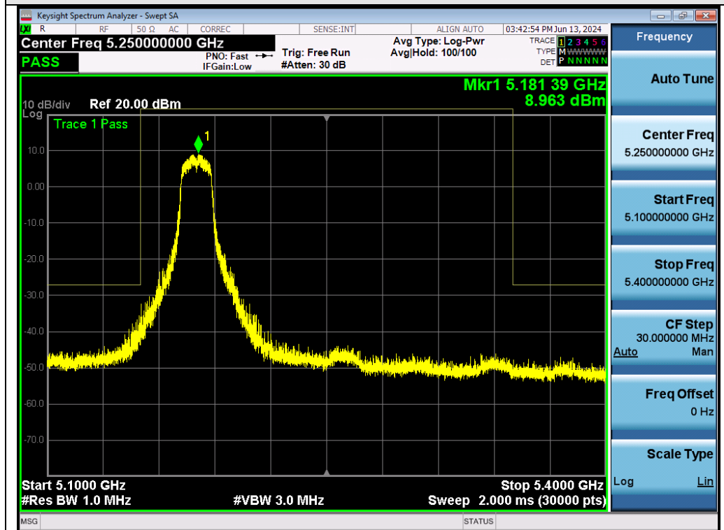
Test_Graph_802.11ac20_CHAIN B_5180_6Mbps_Frequency Band 3
