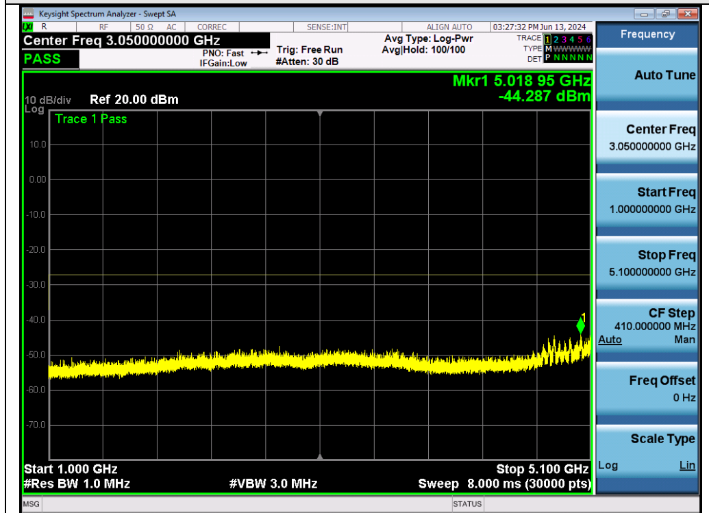
Test_Graph_802.11ac20_CHAIN A_5180_6Mbps_Frequency Band 2
