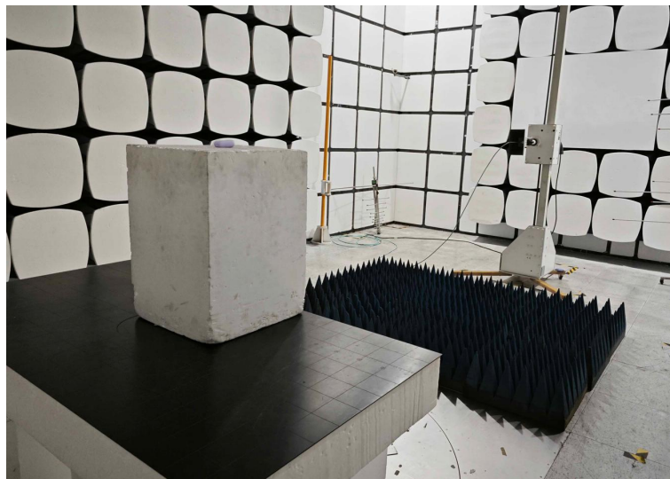
Radiated emission above 1GHz
