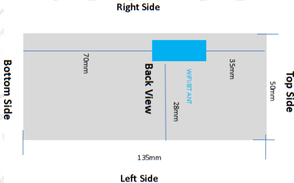
Distance of The Antenna vertical to the EUT surface and edge
